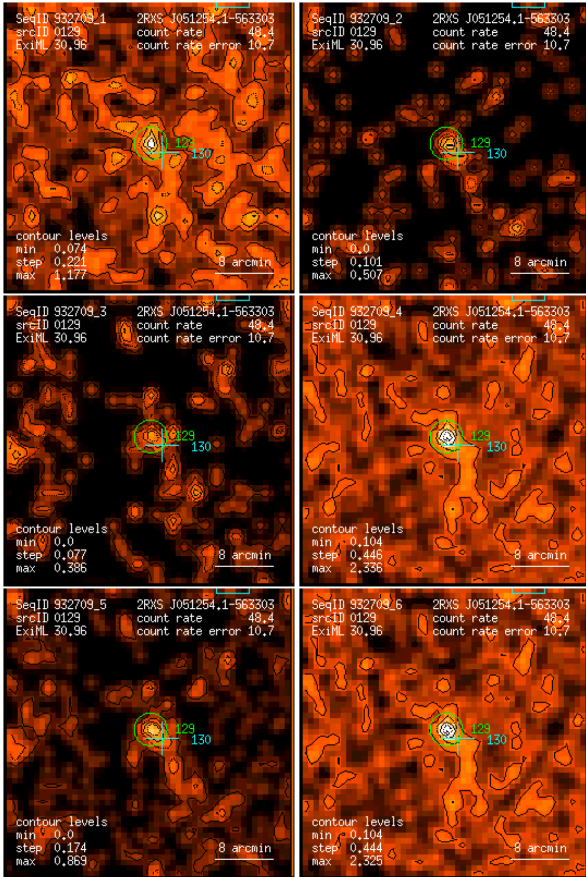
Figure 129: RASS 932709: detection 0129: band rate images, Gaussian filter: (1) PSPC channels 11 – 41, (2) 52 – 90, (3) 91 – 201, (4) 11 – 235, (5) 52 – 201, (6) 11 – 201. Broad band rates in counts/ks. Band rate contour levels in counts/ks/arcmin 2 .
