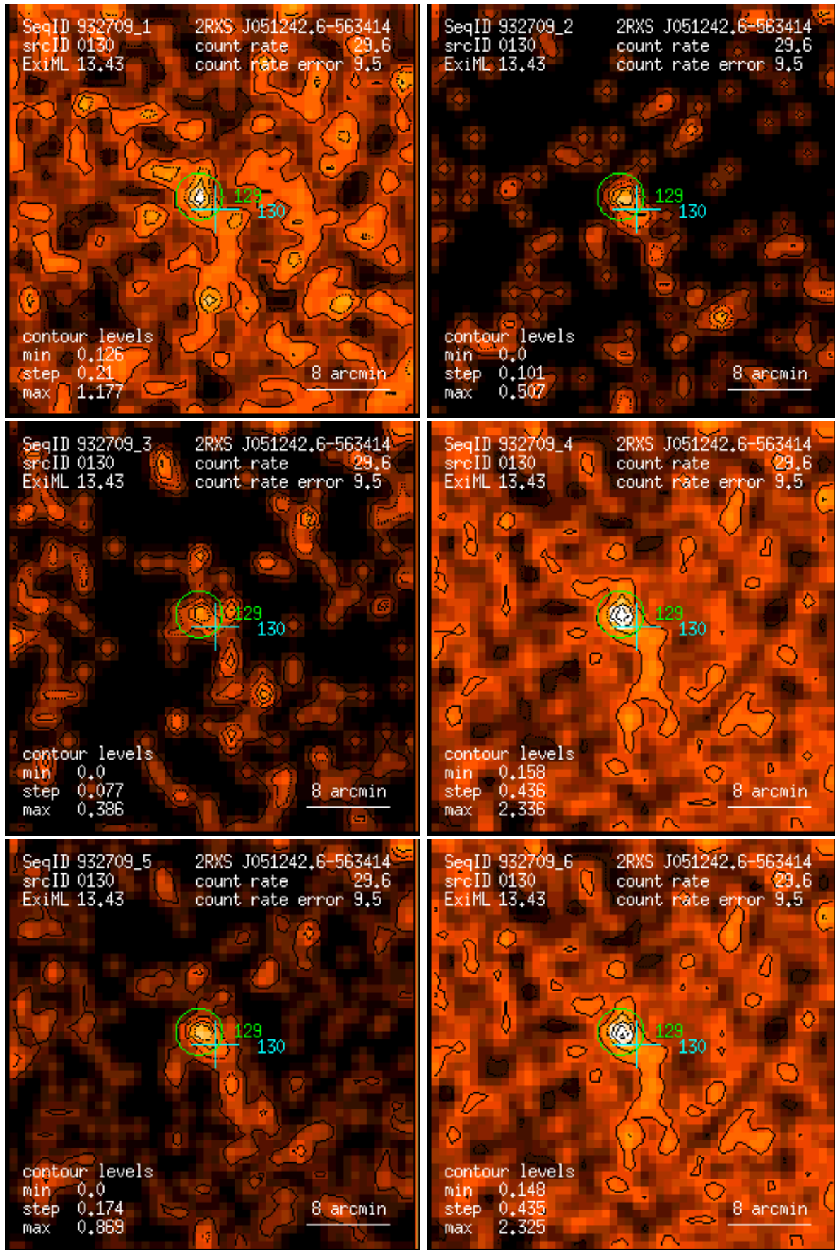
Figure 130: RASS 932709: detection 0130: band rate images, Gaussian filter: (1) PSPC channels 11 – 41, (2) 52 – 90, (3) 91 – 201, (4) 11 – 235, (5) 52 – 201, (6) 11 – 201. Broad band rates in counts/ks. Band rate contour levels in counts/ks/arcmin 2 .
