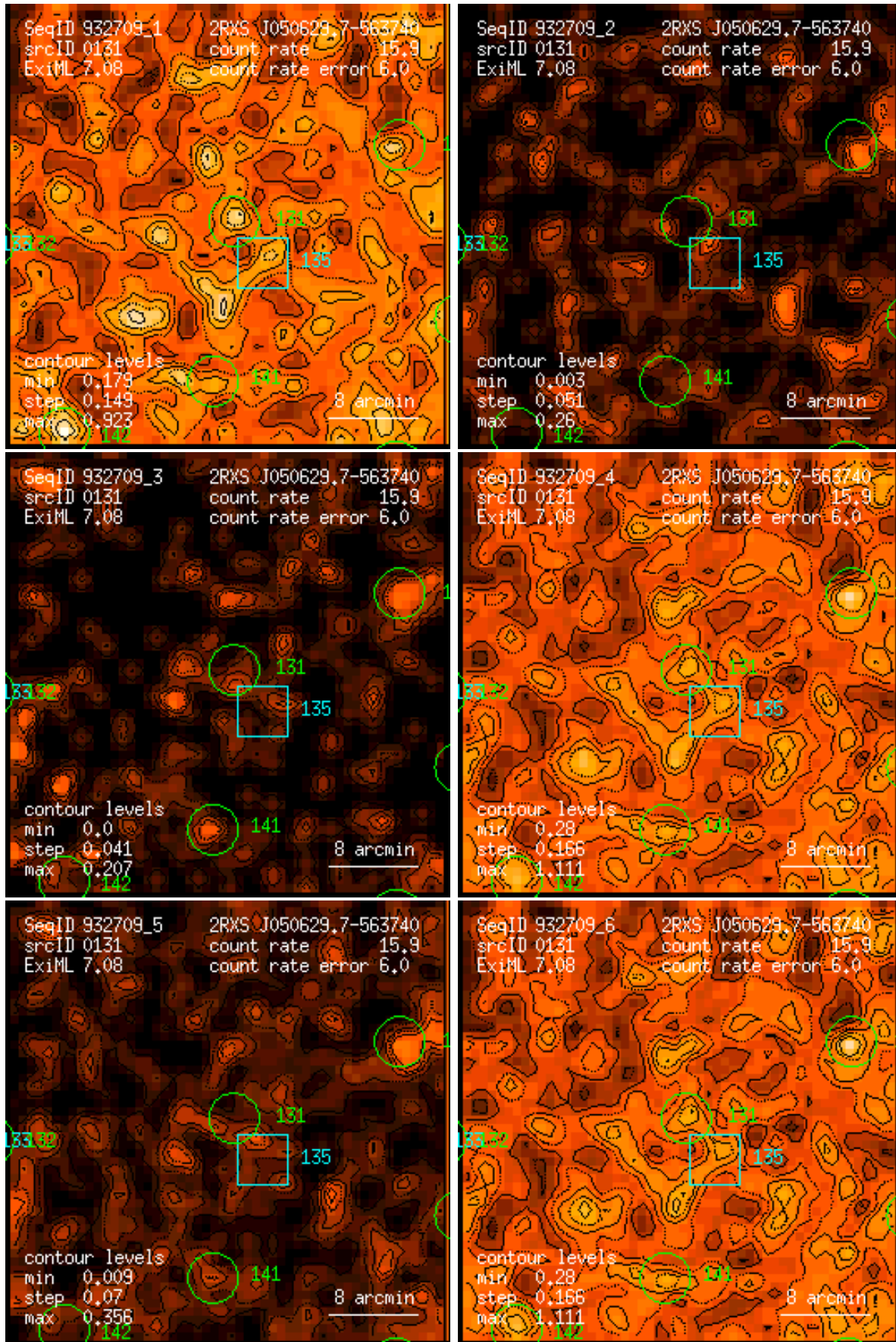
Figure 131: RASS 932709: detection 0131: band rate images, Gaussian filter: (1) PSPC channels 11 – 41, (2) 52 – 90, (3) 91 – 201, (4) 11 – 235, (5) 52 – 201, (6) 11 – 201. Broad band rates in counts/ks. Band rate contour levels in counts/ks/arcmin 2 .
