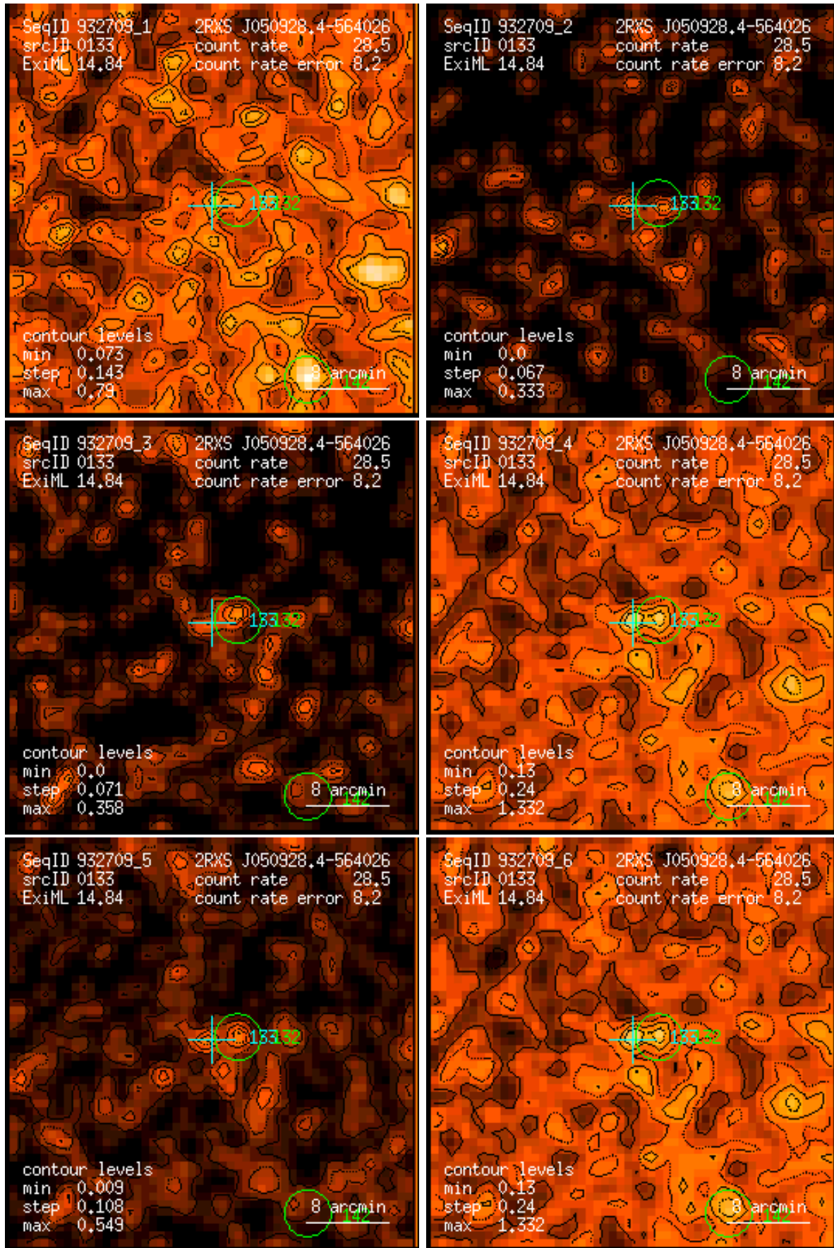
Figure 133: RASS 932709: detection 0133: band rate images, Gaussian filter: (1) PSPC channels 11 – 41, (2) 52 – 90, (3) 91 – 201, (4) 11 – 235, (5) 52 – 201, (6) 11 – 201. Broad band rates in counts/ks. Band rate contour levels in counts/ks/arcmin 2 .
