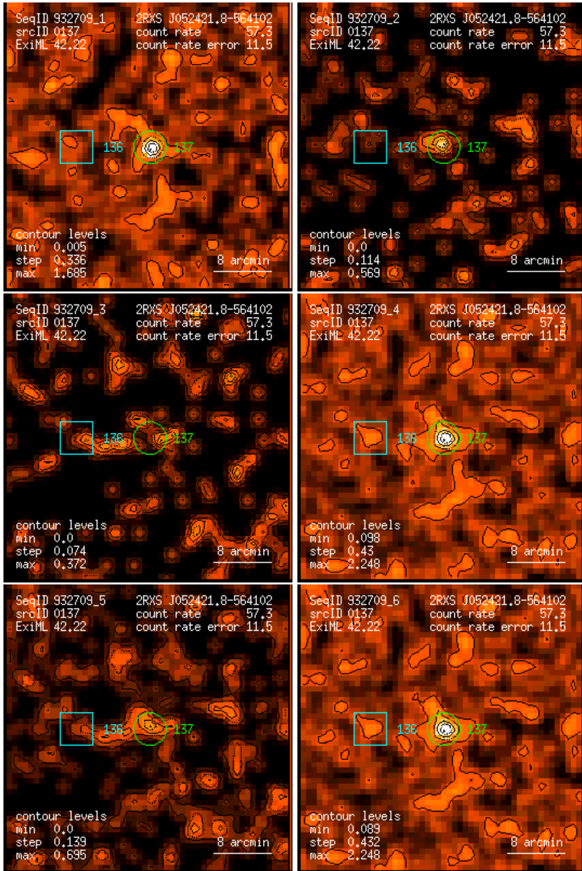
Figure 137: RASS 932709: detection 0137: band rate images, Gaussian filter: (1) PSPC channels 11 – 41, (2) 52 – 90, (3) 91 – 201, (4) 11 – 235, (5) 52 – 201, (6) 11 – 201. Broad band rates in counts/ks. Band rate contour levels in counts/ks/arcmin 2 .
