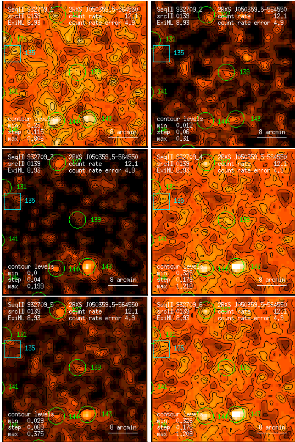
Figure 139: RASS 932709: detection 0139: band rate images, Gaussian filter: (1) PSPC channels 11 – 41, (2) 52 – 90, (3) 91 – 201, (4) 11 – 235, (5) 52 – 201, (6) 11 – 201. Broad band rates in counts/ks. Band rate contour levels in counts/ks/arcmin 2 .
