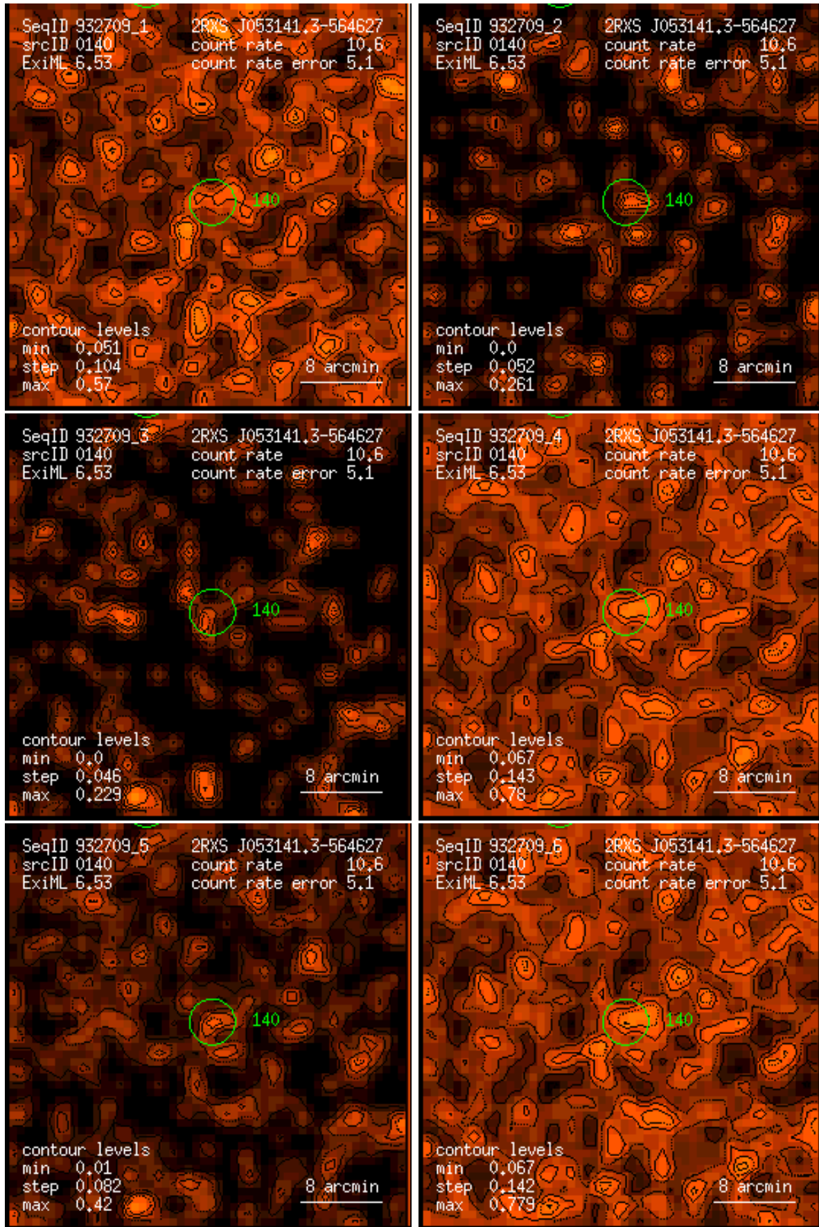
Figure 140: RASS 932709: detection 0140: band rate images, Gaussian filter: (1) PSPC channels 11 – 41, (2) 52 – 90, (3) 91 – 201, (4) 11 – 235, (5) 52 – 201, (6) 11 – 201. Broad band rates in counts/ks. Band rate contour levels in counts/ks/arcmin 2 .
