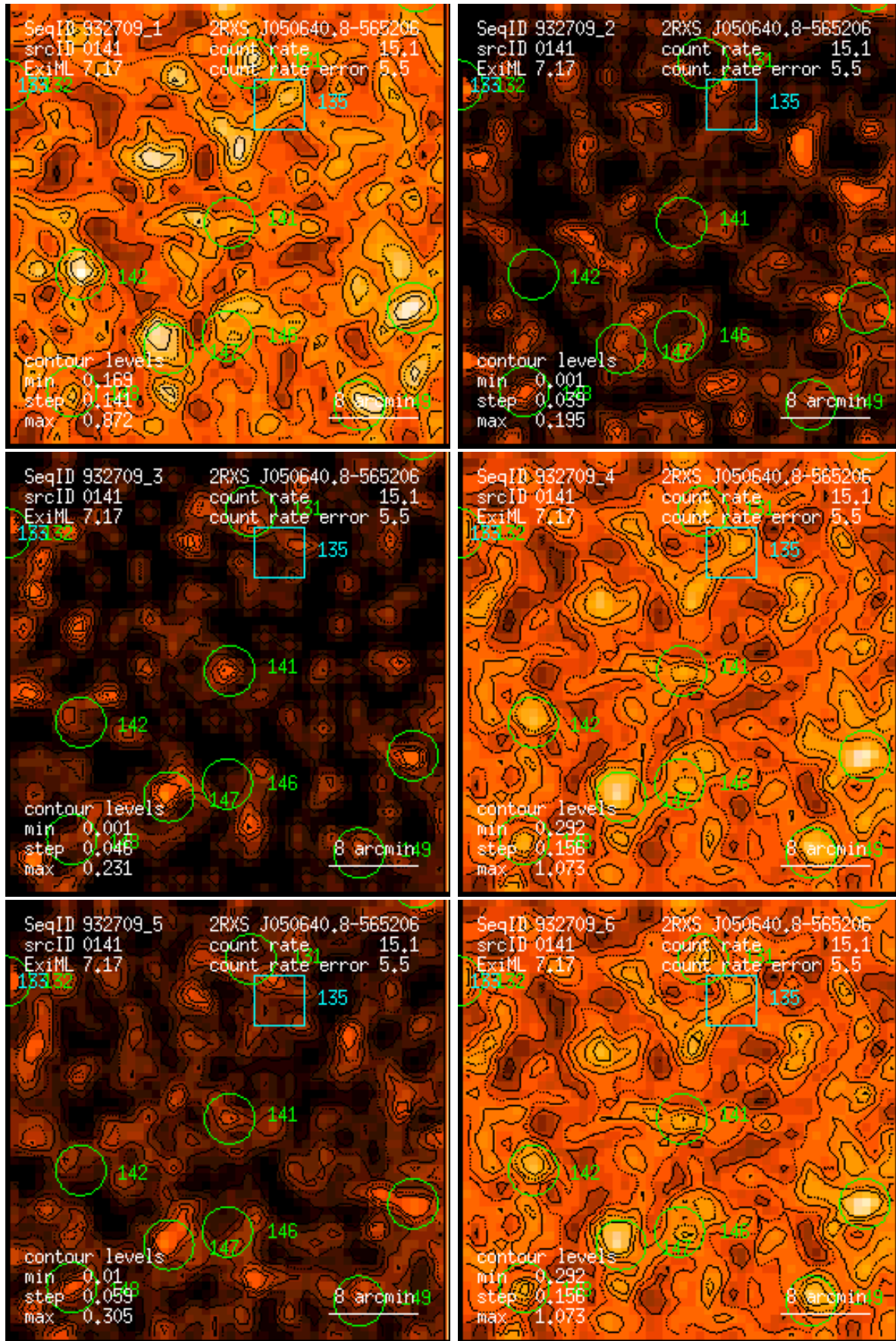
Figure 141: RASS 932709: detection 0141: band rate images, Gaussian filter: (1) PSPC channels 11 – 41, (2) 52 – 90, (3) 91 – 201, (4) 11 – 235, (5) 52 – 201, (6) 11 – 201. Broad band rates in counts/ks. Band rate contour levels in counts/ks/arcmin 2 .
