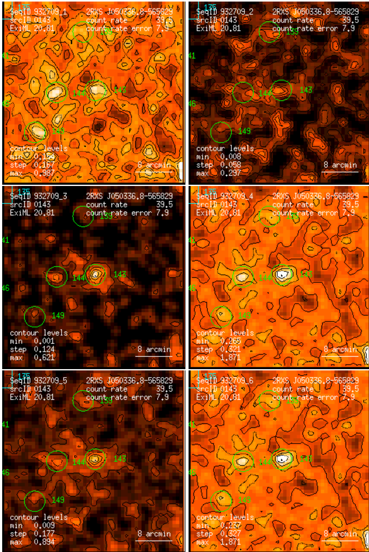
Figure 143: RASS 932709: detection 0143: band rate images, Gaussian filter: (1) PSPC channels 11 – 41, (2) 52 – 90, (3) 91 – 201, (4) 11 – 235, (5) 52 – 201, (6) 11 – 201. Broad band rates in counts/ks. Band rate contour levels in counts/ks/arcmin 2 .
