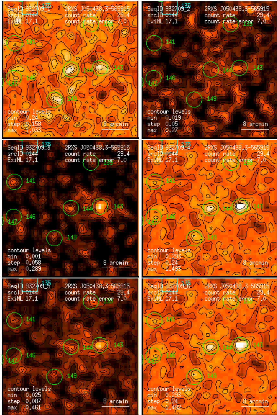
Figure 144: RASS 932709: detection 0144: band rate images, Gaussian filter: (1) PSPC channels 11 – 41, (2) 52 – 90, (3) 91 – 201, (4) 11 – 235, (5) 52 – 201, (6) 11 – 201. Broad band rates in counts/ks. Band rate contour levels in counts/ks/arcmin 2 .
