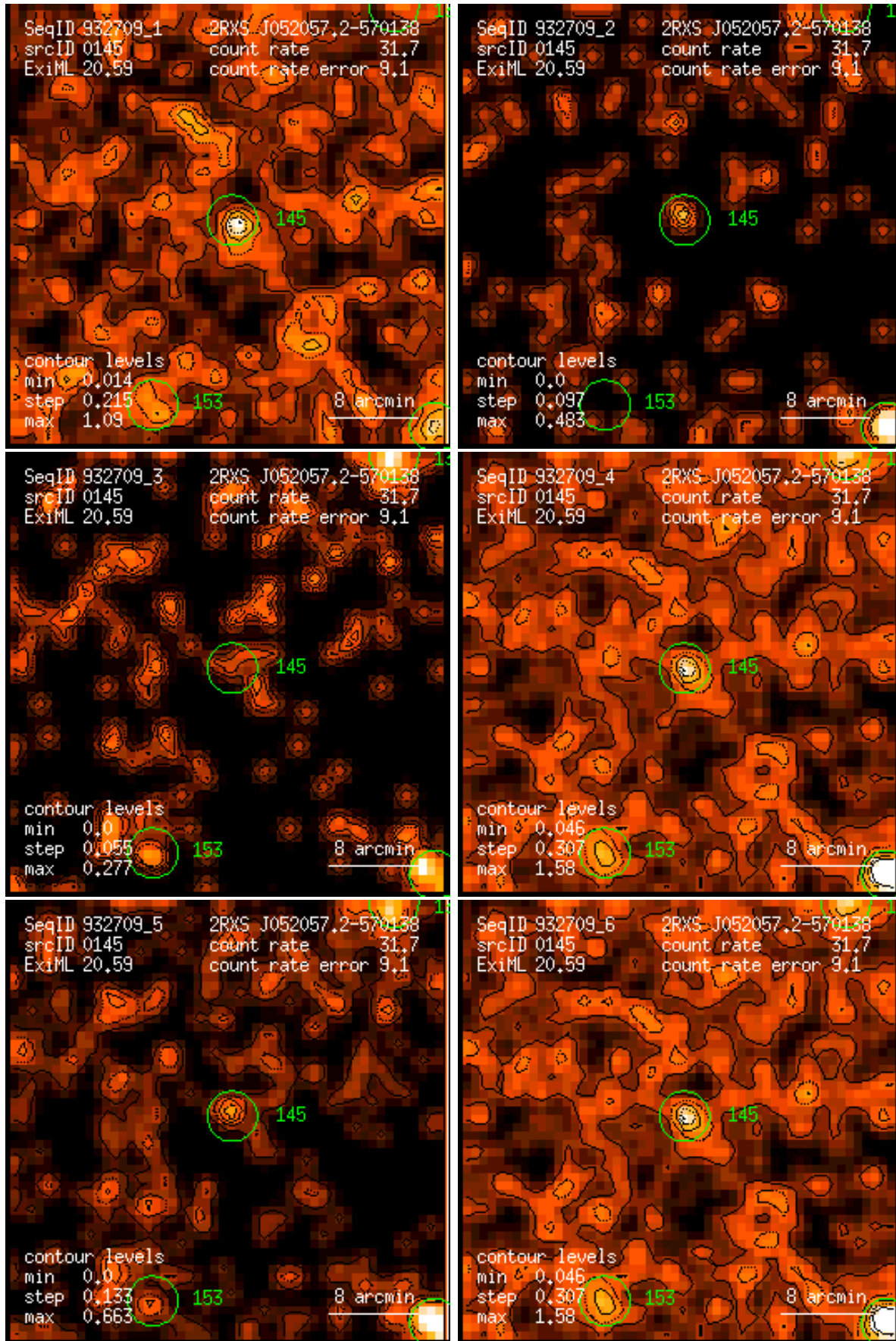
Figure 145: RASS 932709: detection 0145: band rate images, Gaussian filter: (1) PSPC channels 11 – 41, (2) 52 – 90, (3) 91 – 201, (4) 11 – 235, (5) 52 – 201, (6) 11 – 201. Broad band rates in counts/ks. Band rate contour levels in counts/ks/arcmin 2 .
