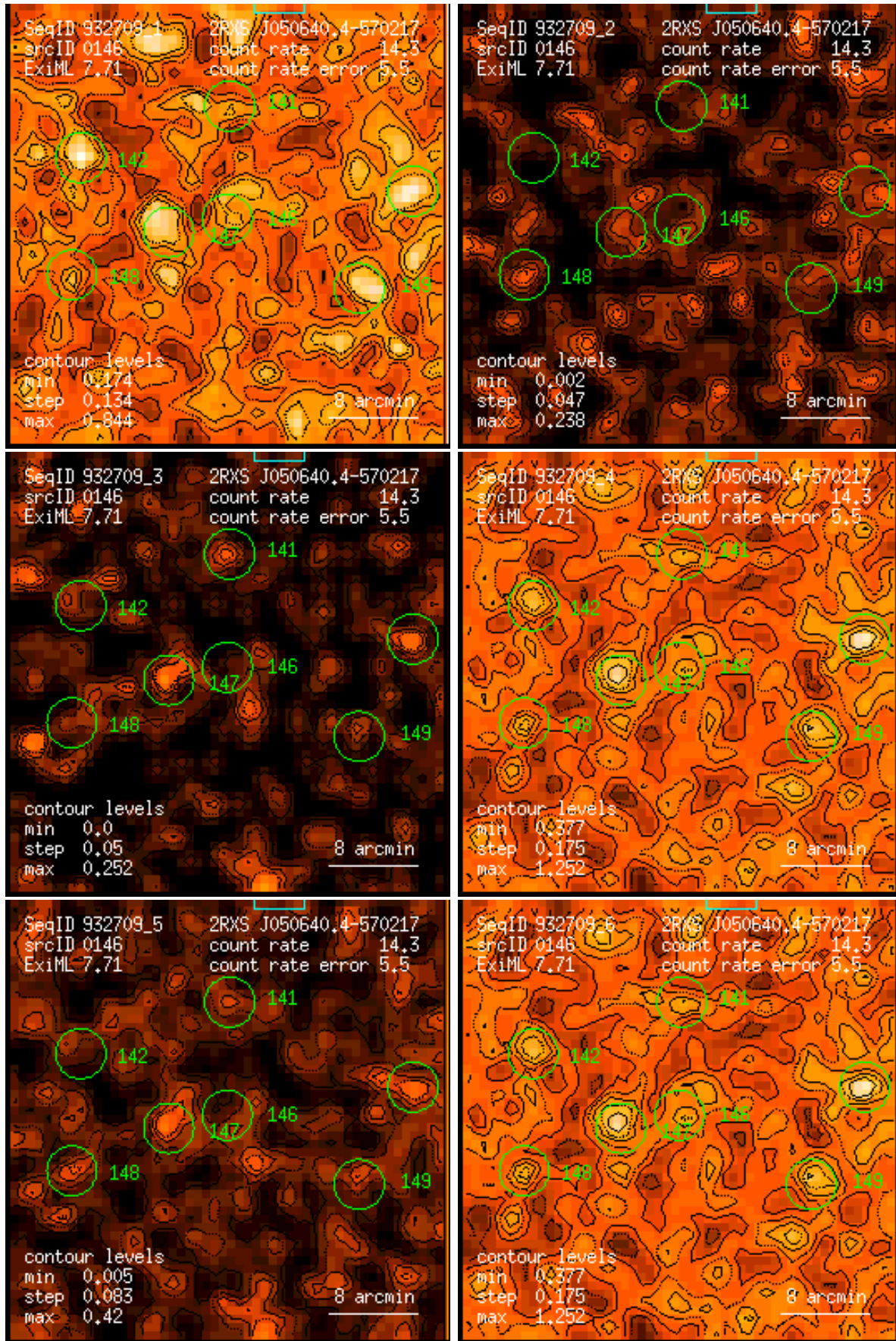
Figure 146: RASS 932709: detection 0146: band rate images, Gaussian filter: (1) PSPC channels 11 – 41, (2) 52 – 90, (3) 91 – 201, (4) 11 – 235, (5) 52 – 201, (6) 11 – 201. Broad band rates in counts/ks. Band rate contour levels in counts/ks/arcmin 2 .
