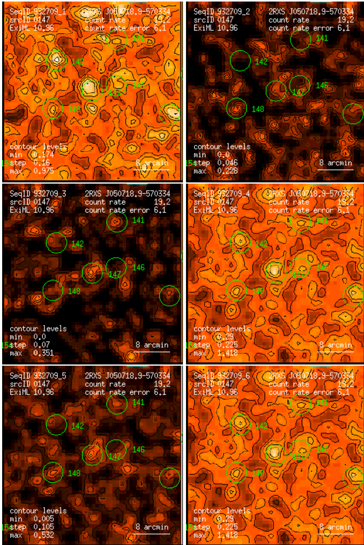
Figure 147: RASS 932709: detection 0147: band rate images, Gaussian filter: (1) PSPC channels 11 – 41, (2) 52 – 90, (3) 91 – 201, (4) 11 – 235, (5) 52 – 201, (6) 11 – 201. Broad band rates in counts/ks. Band rate contour levels in counts/ks/arcmin 2 .
