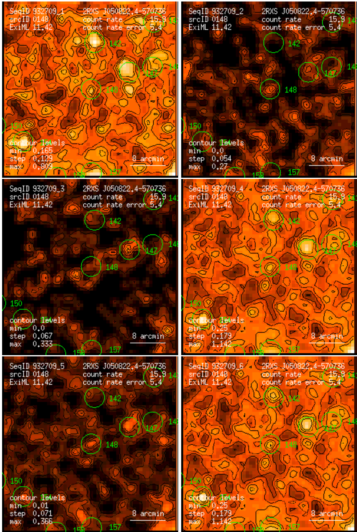
Figure 148: RASS 932709: detection 0148: band rate images, Gaussian filter: (1) PSPC channels 11 – 41, (2) 52 – 90, (3) 91 – 201, (4) 11 – 235, (5) 52 – 201, (6) 11 – 201. Broad band rates in counts/ks. Band rate contour levels in counts/ks/arcmin 2 .
