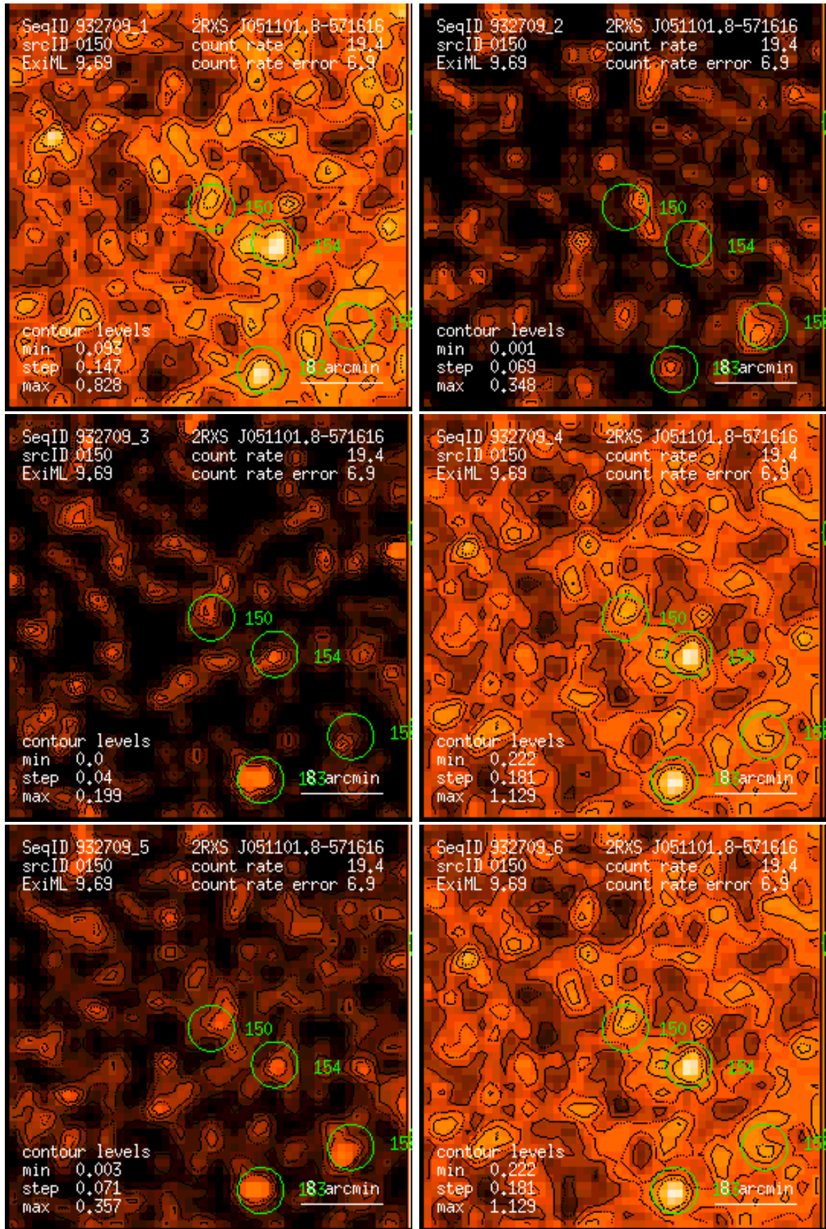
Figure 150: RASS 932709: detection 0150: band rate images, Gaussian filter: (1) PSPC channels 11 – 41, (2) 52 – 90, (3) 91 – 201, (4) 11 – 235, (5) 52 – 201, (6) 11 – 201. Broad band rates in counts/ks. Band rate contour levels in counts/ks/arcmin 2 .
