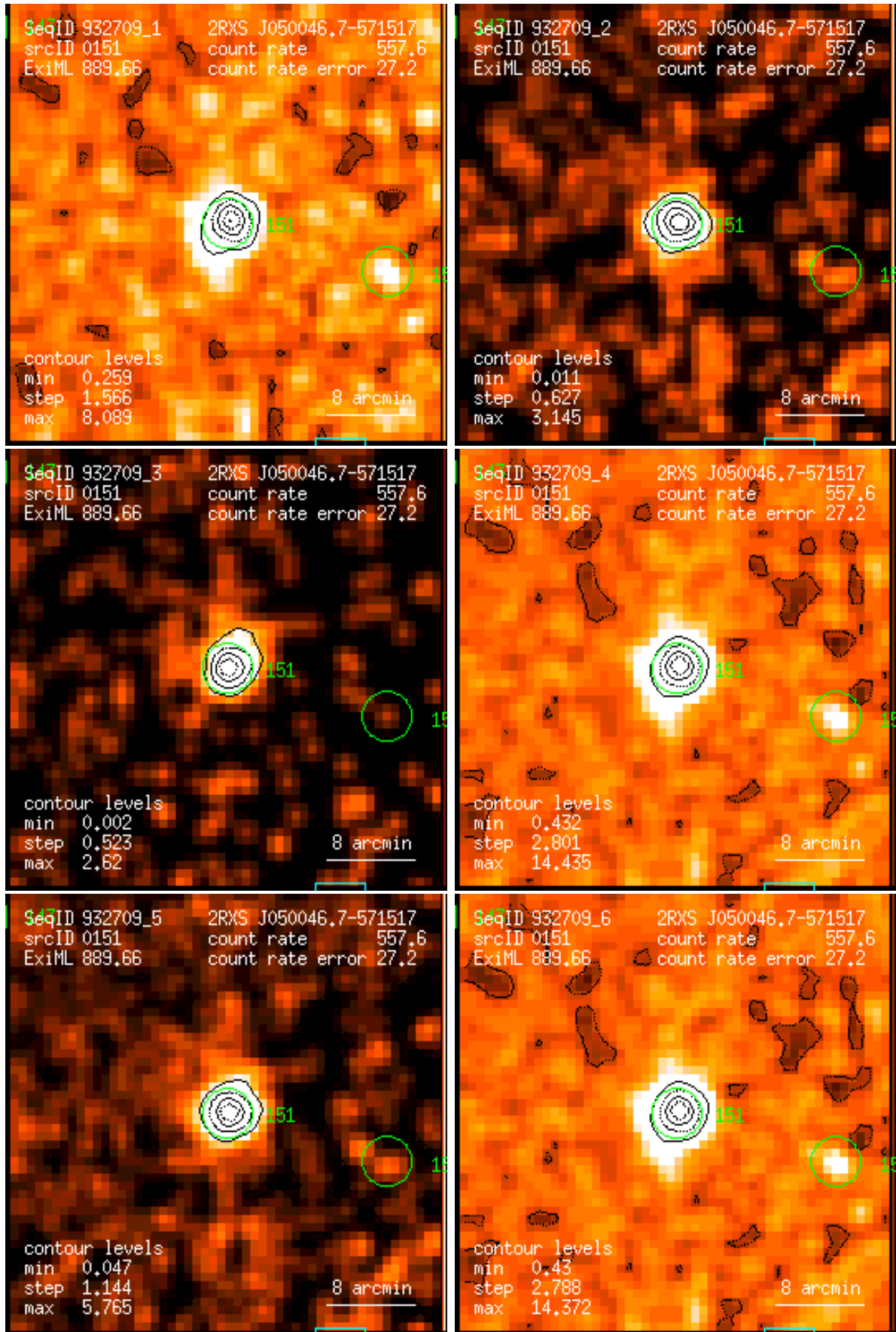
Figure 151: RASS 932709: detection 0151: band rate images, Gaussian filter: (1) PSPC channels 11 – 41, (2) 52 – 90, (3) 91 – 201, (4) 11 – 235, (5) 52 – 201, (6) 11 – 201. Broad band rates in counts/ks. Band rate contour levels in counts/ks/arcmin 2 .
