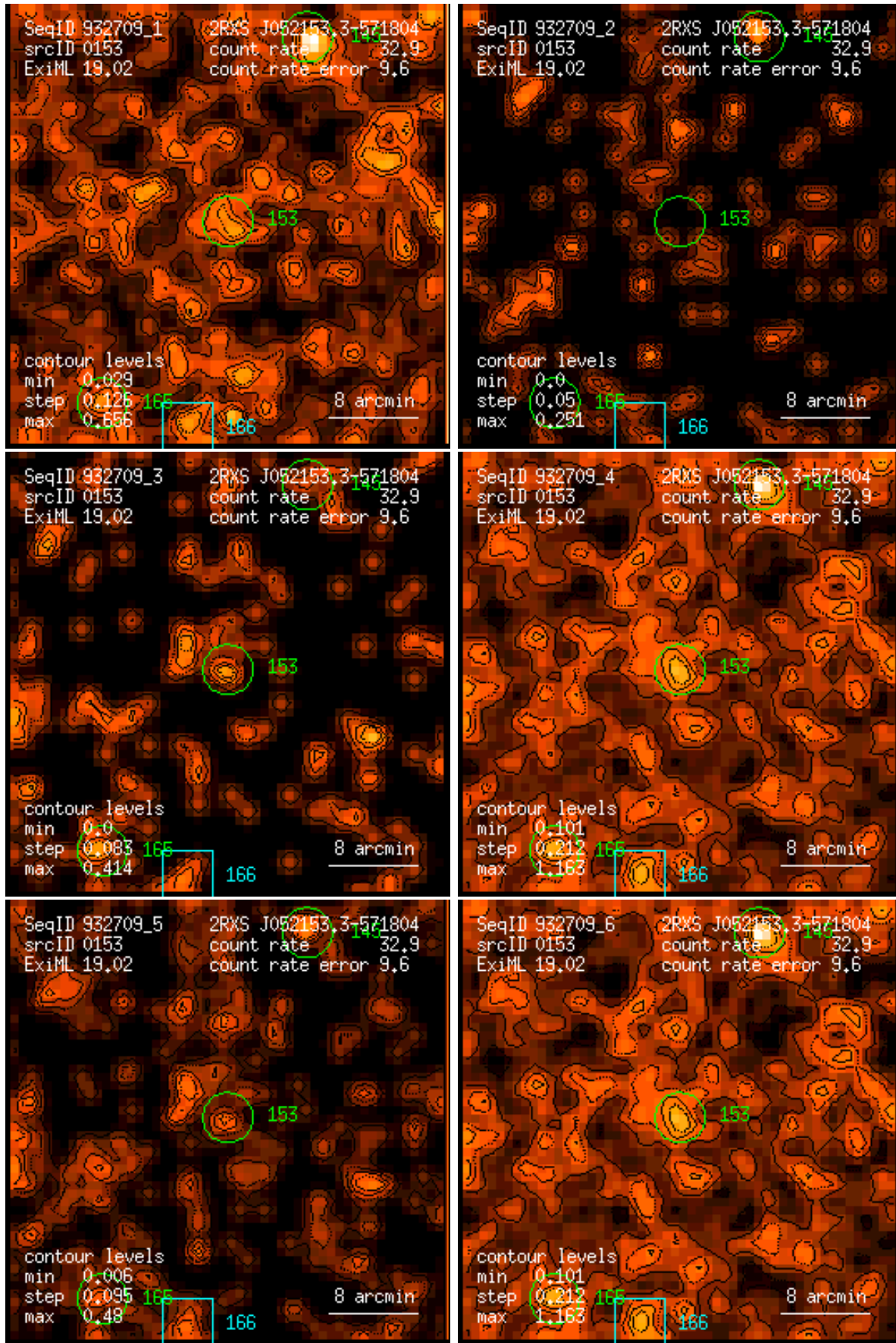
Figure 153: RASS 932709: detection 0153: band rate images, Gaussian filter: (1) PSPC channels 11 – 41, (2) 52 – 90, (3) 91 – 201, (4) 11 – 235, (5) 52 – 201, (6) 11 – 201. Broad band rates in counts/ks. Band rate contour levels in counts/ks/arcmin 2 .
