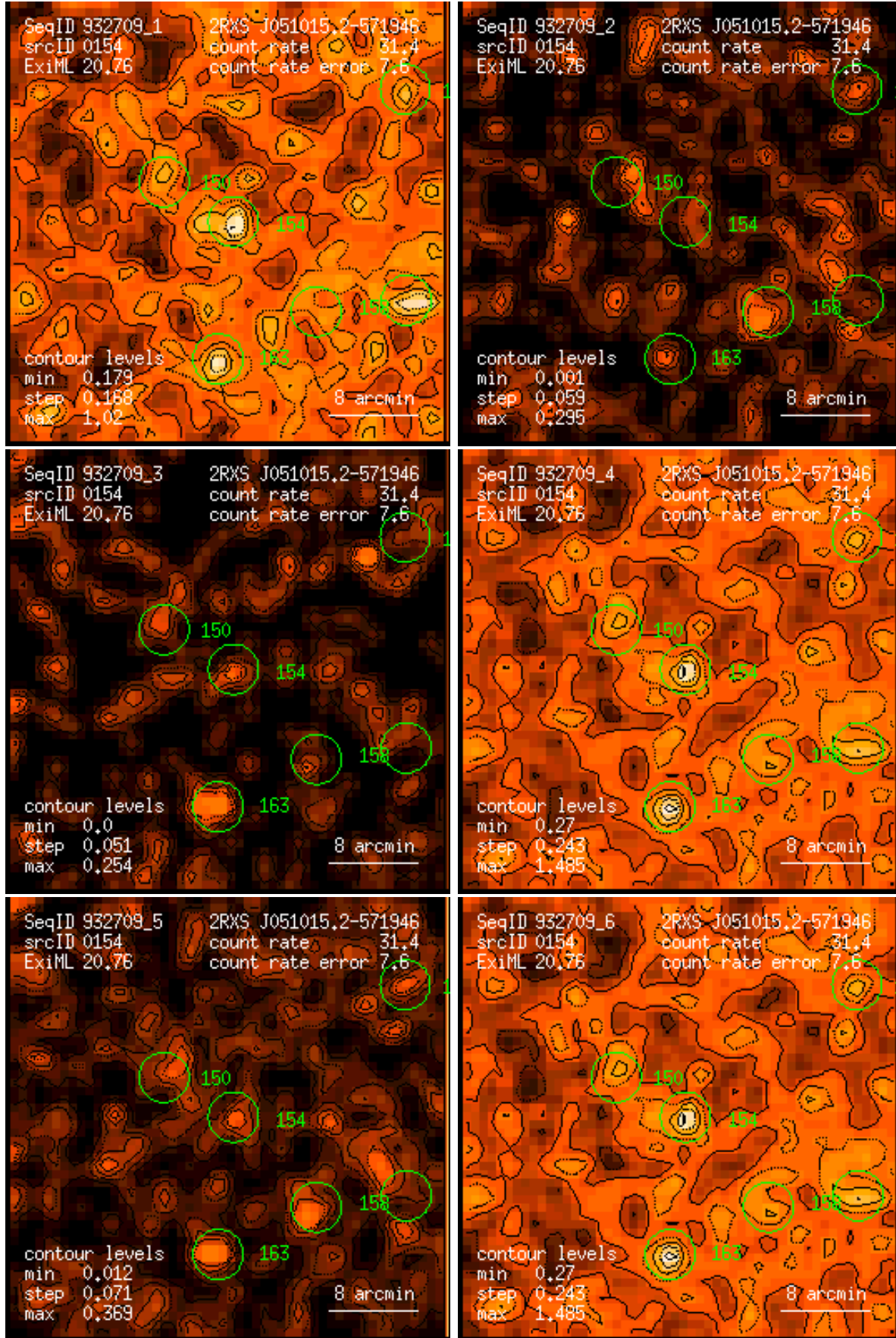
Figure 154: RASS 932709: detection 0154: band rate images, Gaussian filter: (1) PSPC channels 11 – 41, (2) 52 – 90, (3) 91 – 201, (4) 11 – 235, (5) 52 – 201, (6) 11 – 201. Broad band rates in counts/ks. Band rate contour levels in counts/ks/arcmin 2 .
