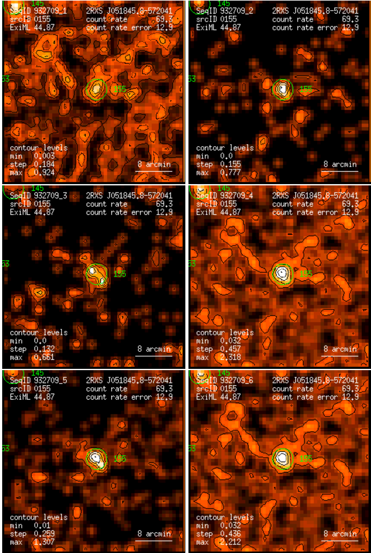
Figure 155: RASS 932709: detection 0155: band rate images, Gaussian filter: (1) PSPC channels 11 – 41, (2) 52 – 90, (3) 91 – 201, (4) 11 – 235, (5) 52 – 201, (6) 11 – 201. Broad band rates in counts/ks. Band rate contour levels in counts/ks/arcmin 2 .
