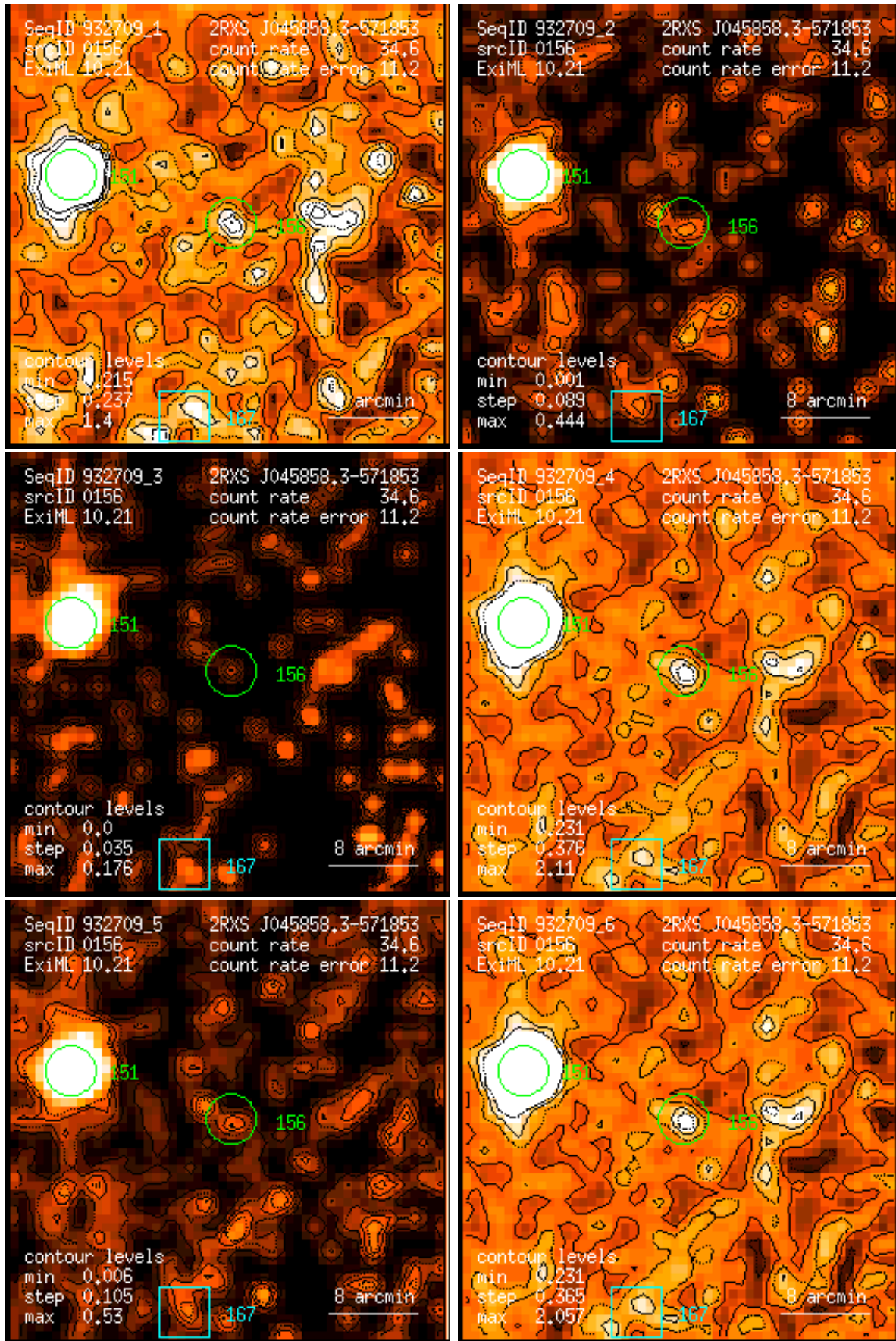
Figure 156: RASS 932709: detection 0156: band rate images, Gaussian filter: (1) PSPC channels 11 – 41, (2) 52 – 90, (3) 91 – 201, (4) 11 – 235, (5) 52 – 201, (6) 11 – 201. Broad band rates in counts/ks. Band rate contour levels in counts/ks/arcmin 2 .
