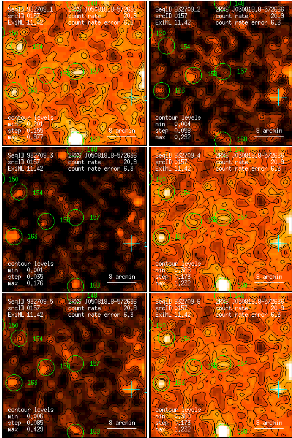
Figure 157: RASS 932709: detection 0157: band rate images, Gaussian filter: (1) PSPC channels 11 – 41, (2) 52 – 90, (3) 91 – 201, (4) 11 – 235, (5) 52 – 201, (6) 11 – 201. Broad band rates in counts/ks. Band rate contour levels in counts/ks/arcmin 2 .
