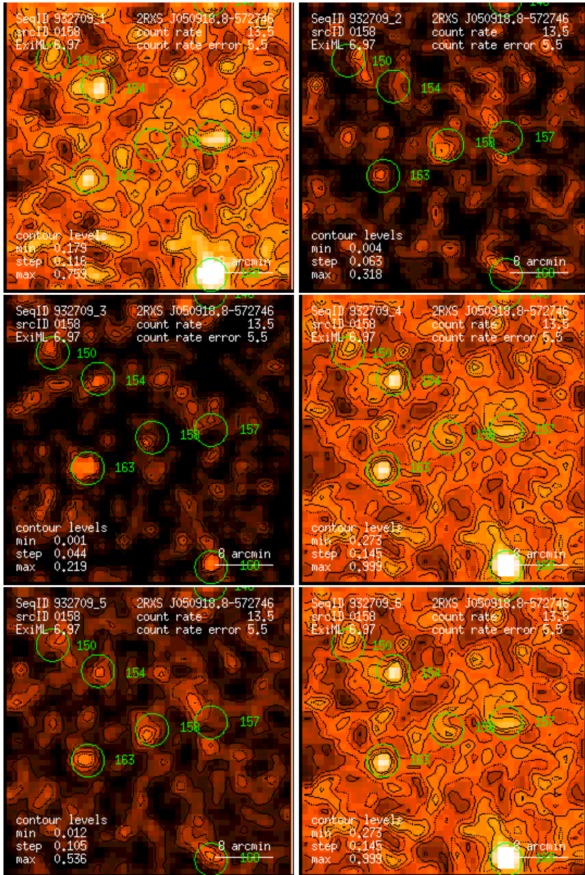
Figure 158: RASS 932709: detection 0158: band rate images, Gaussian filter: (1) PSPC channels 11 – 41, (2) 52 – 90, (3) 91 – 201, (4) 11 – 235, (5) 52 – 201, (6) 11 – 201. Broad band rates in counts/ks. Band rate contour levels in counts/ks/arcmin 2 .
