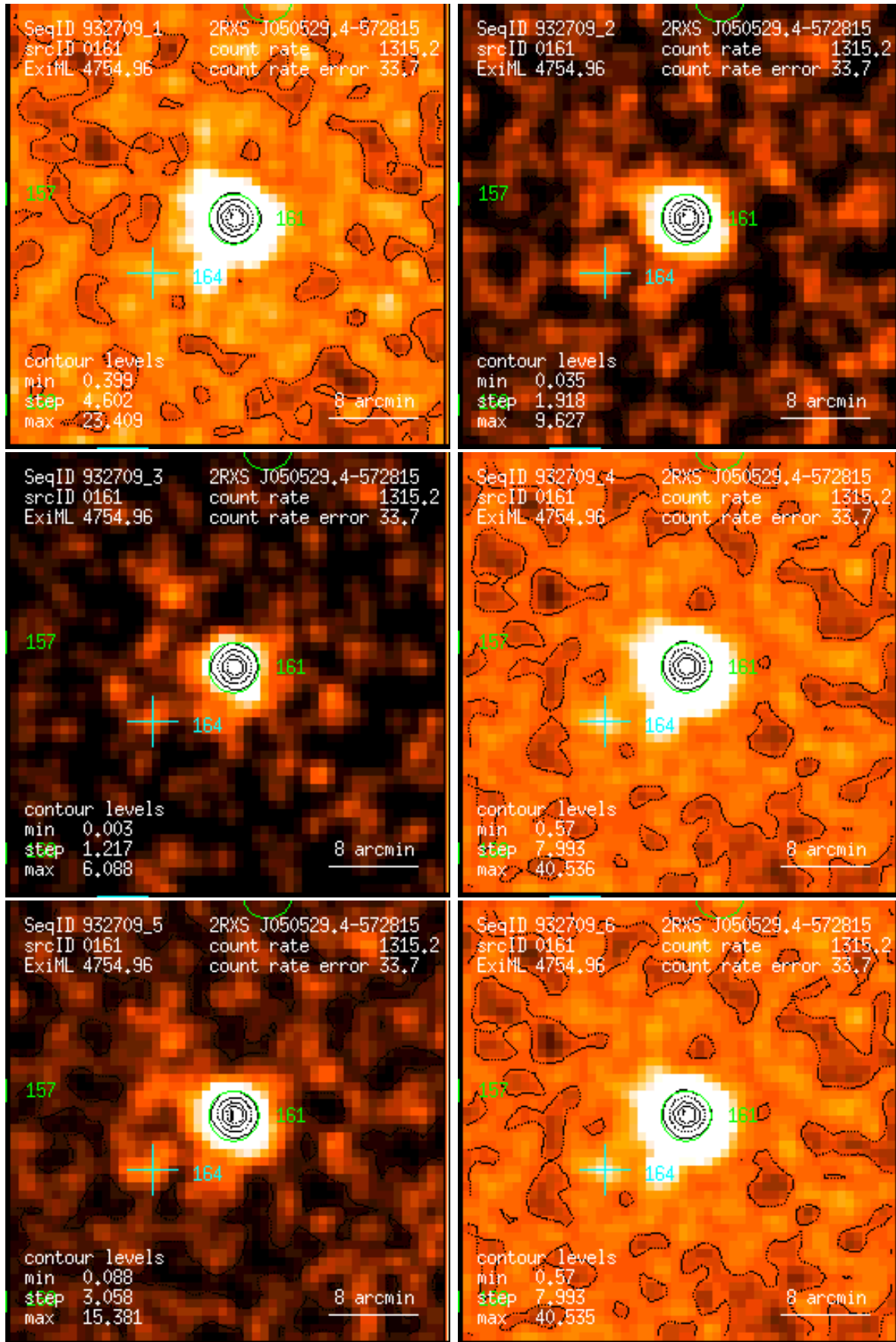
Figure 161: RASS 932709: detection 0161: band rate images, Gaussian filter: (1) PSPC channels 11 – 41, (2) 52 – 90, (3) 91 – 201, (4) 11 – 235, (5) 52 – 201, (6) 11 – 201. Broad band rates in counts/ks. Band rate contour levels in counts/ks/arcmin 2 .
