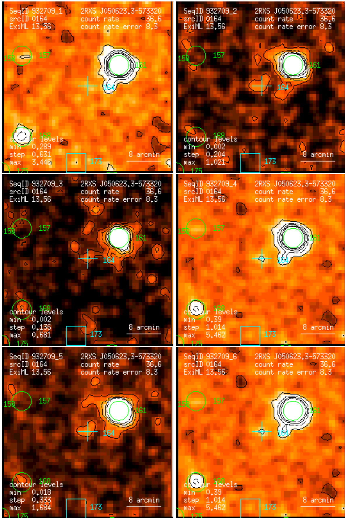
Figure 164: RASS 932709: detection 0164: band rate images, Gaussian filter: (1) PSPC channels 11 – 41, (2) 52 – 90, (3) 91 – 201, (4) 11 – 235, (5) 52 – 201, (6) 11 – 201. Broad band rates in counts/ks. Band rate contour levels in counts/ks/arcmin 2 .
