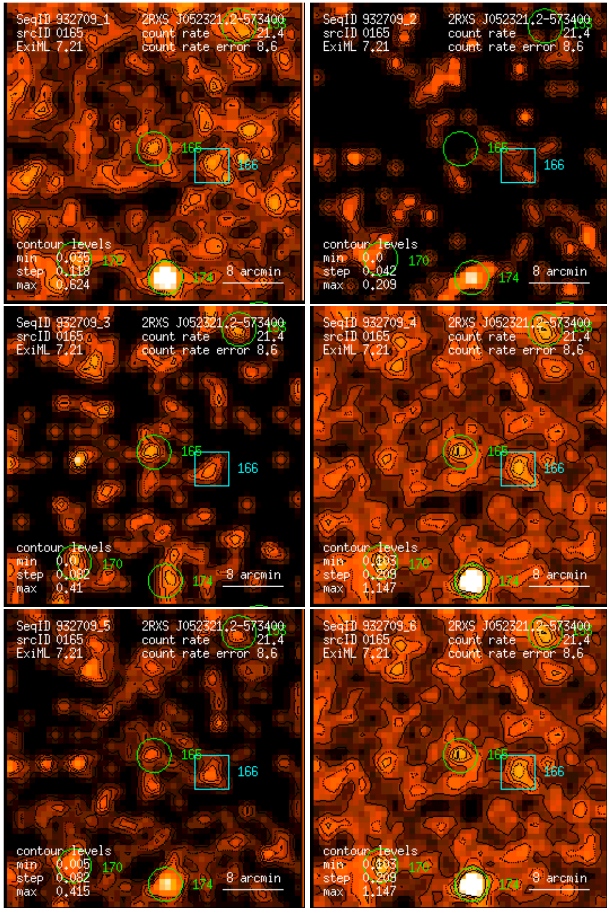
Figure 165: RASS 932709: detection 0165: band rate images, Gaussian filter: (1) PSPC channels 11 – 41, (2) 52 – 90, (3) 91 – 201, (4) 11 – 235, (5) 52 – 201, (6) 11 – 201. Broad band rates in counts/ks. Band rate contour levels in counts/ks/arcmin 2 .
