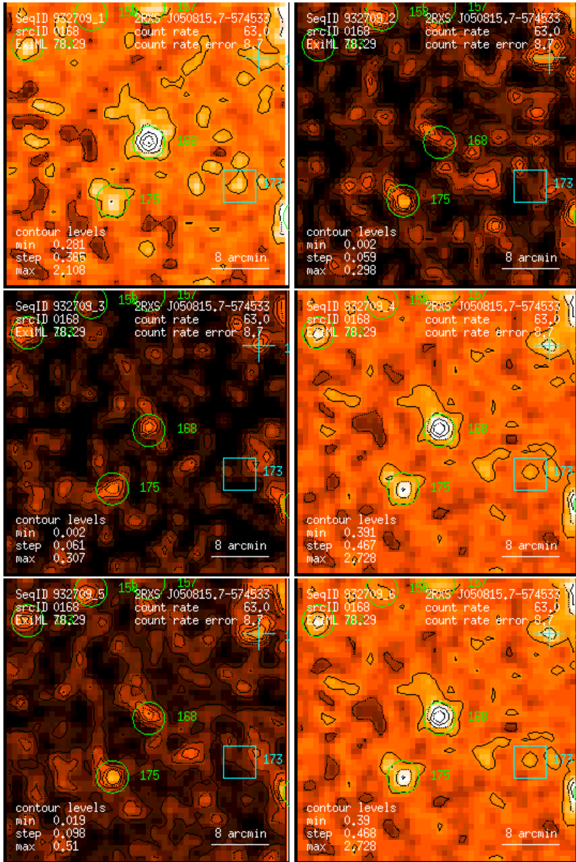
Figure 168: RASS 932709: detection 0168: band rate images, Gaussian filter: (1) PSPC channels 11 – 41, (2) 52 – 90, (3) 91 – 201, (4) 11 – 235, (5) 52 – 201, (6) 11 – 201. Broad band rates in counts/ks. Band rate contour levels in counts/ks/arcmin 2 .
