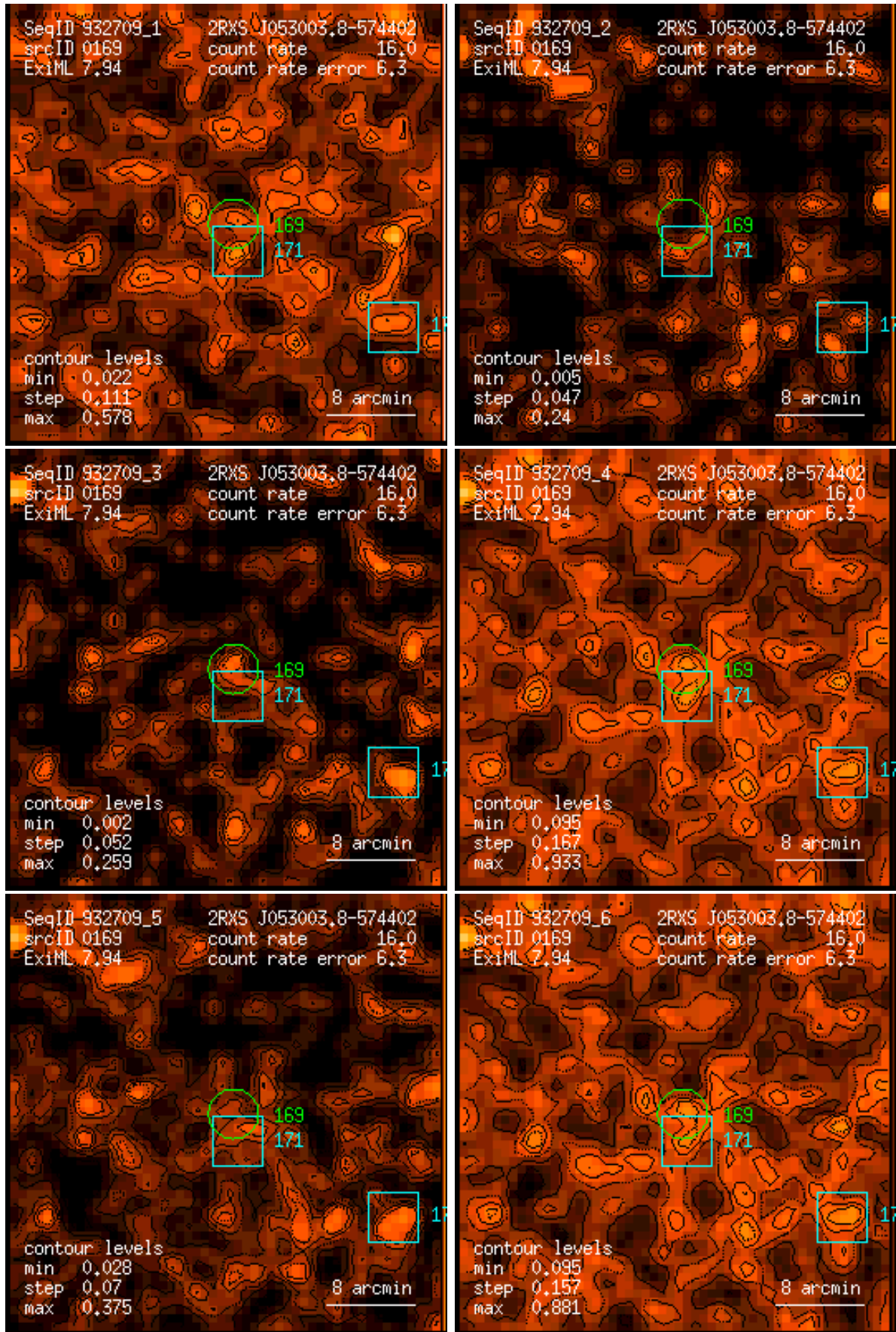
Figure 169: RASS 932709: detection 0169: band rate images, Gaussian filter: (1) PSPC channels 11 – 41, (2) 52 – 90, (3) 91 – 201, (4) 11 – 235, (5) 52 – 201, (6) 11 – 201. Broad band rates in counts/ks. Band rate contour levels in counts/ks/arcmin 2 .
