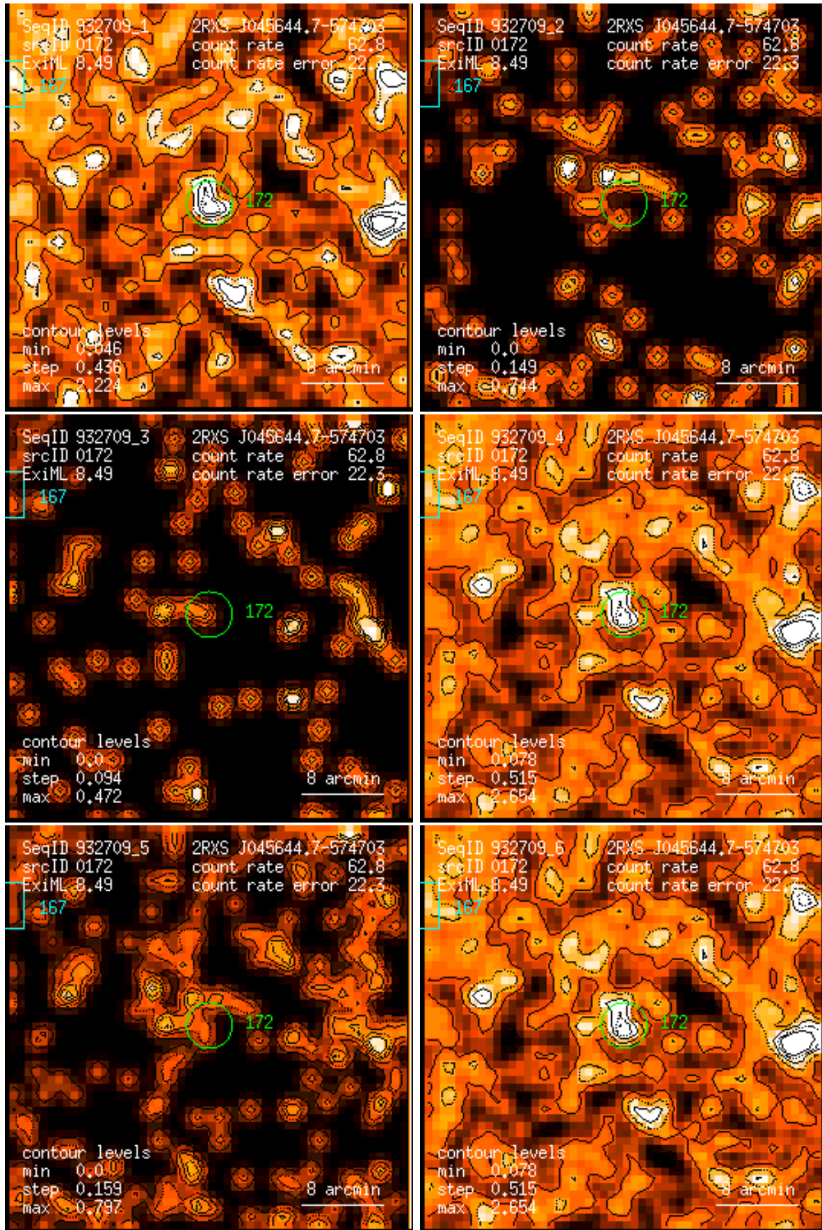
Figure 172: RASS 932709: detection 0172: band rate images, Gaussian filter: (1) PSPC channels 11 – 41, (2) 52 – 90, (3) 91 – 201, (4) 11 – 235, (5) 52 – 201, (6) 11 – 201. Broad band rates in counts/ks. Band rate contour levels in counts/ks/arcmin 2 .
