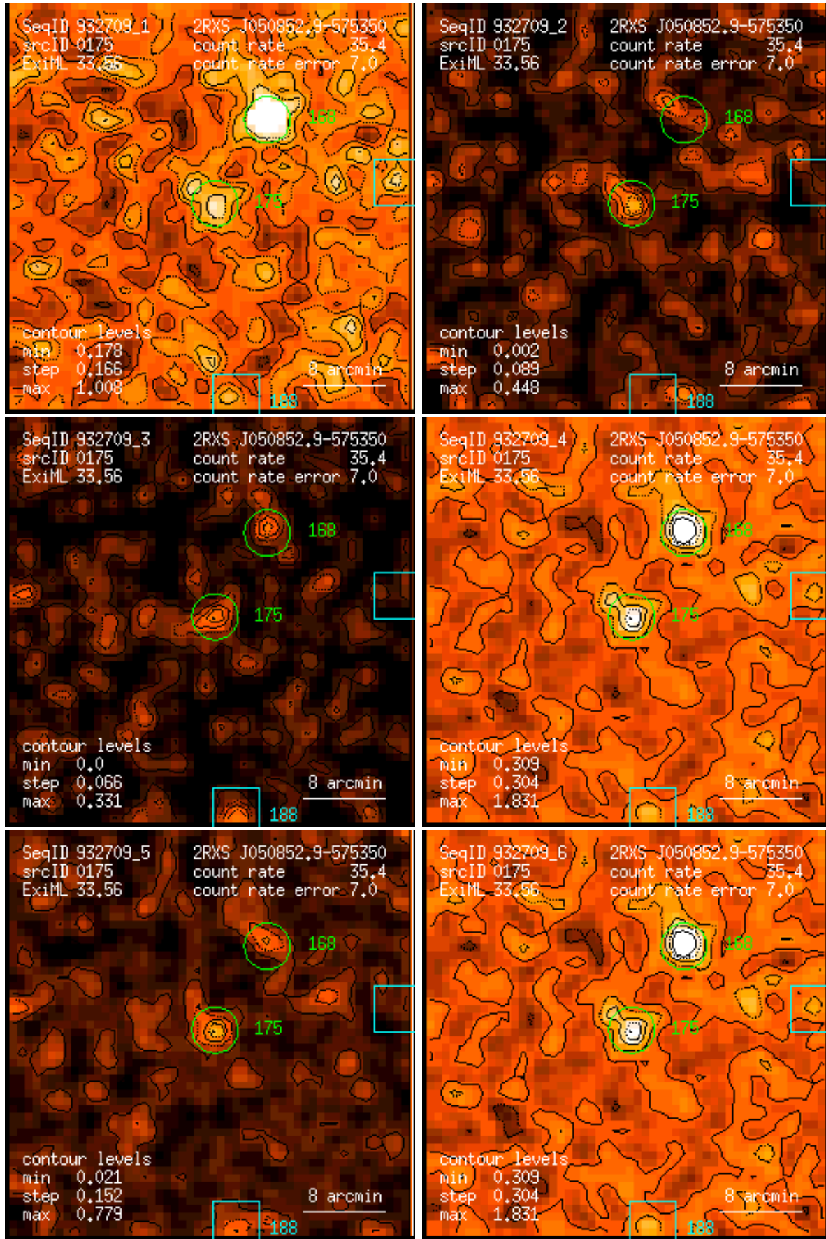
Figure 175: RASS 932709: detection 0175: band rate images, Gaussian filter: (1) PSPC channels 11 – 41, (2) 52 – 90, (3) 91 – 201, (4) 11 – 235, (5) 52 – 201, (6) 11 – 201. Broad band rates in counts/ks. Band rate contour levels in counts/ks/arcmin 2 .
