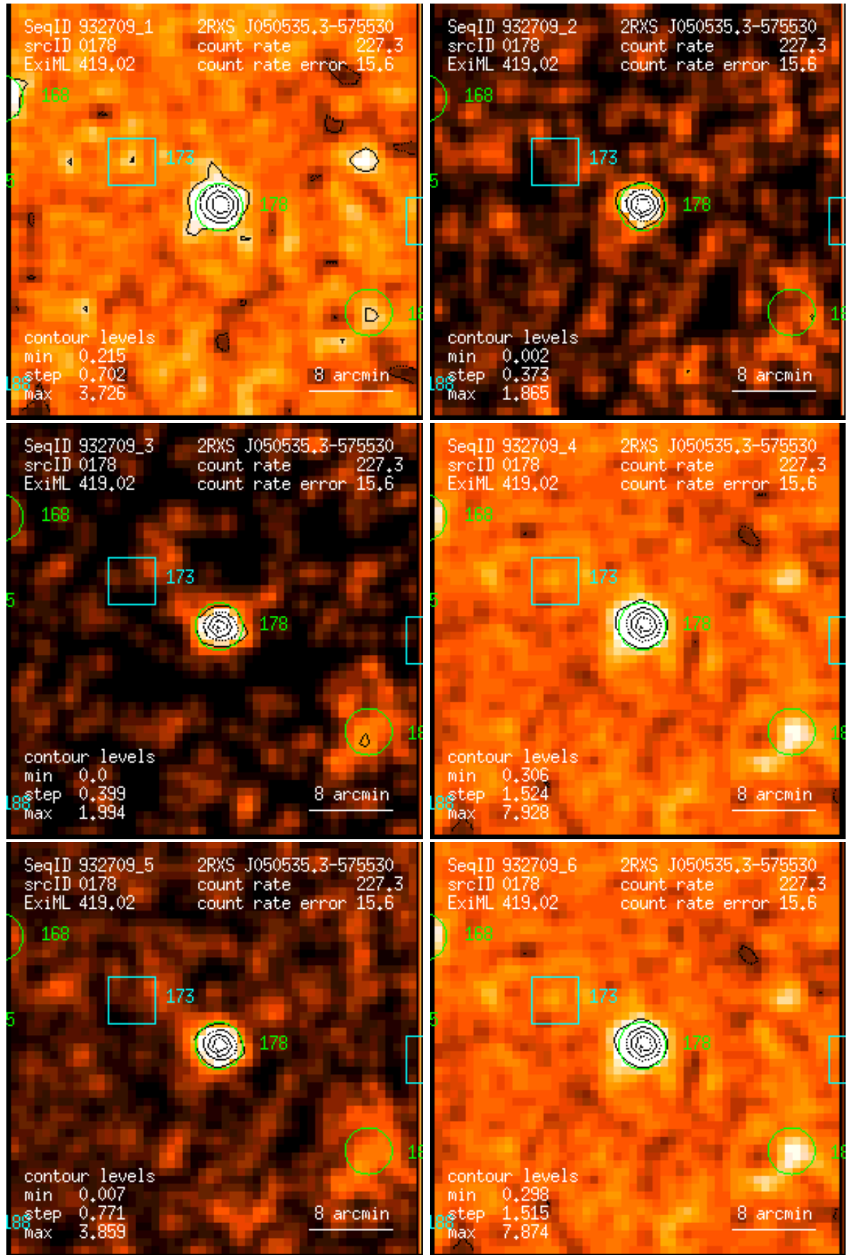
Figure 178: RASS 932709: detection 0178: band rate images, Gaussian filter: (1) PSPC channels 11 – 41, (2) 52 – 90, (3) 91 – 201, (4) 11 – 235, (5) 52 – 201, (6) 11 – 201. Broad band rates in counts/ks. Band rate contour levels in counts/ks/arcmin 2 .
