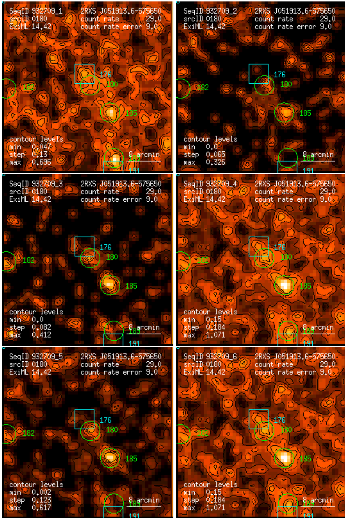
Figure 180: RASS 932709: detection 0180: band rate images, Gaussian filter: (1) PSPC channels 11 – 41, (2) 52 – 90, (3) 91 – 201, (4) 11 – 235, (5) 52 – 201, (6) 11 – 201. Broad band rates in counts/ks. Band rate contour levels in counts/ks/arcmin 2 .
