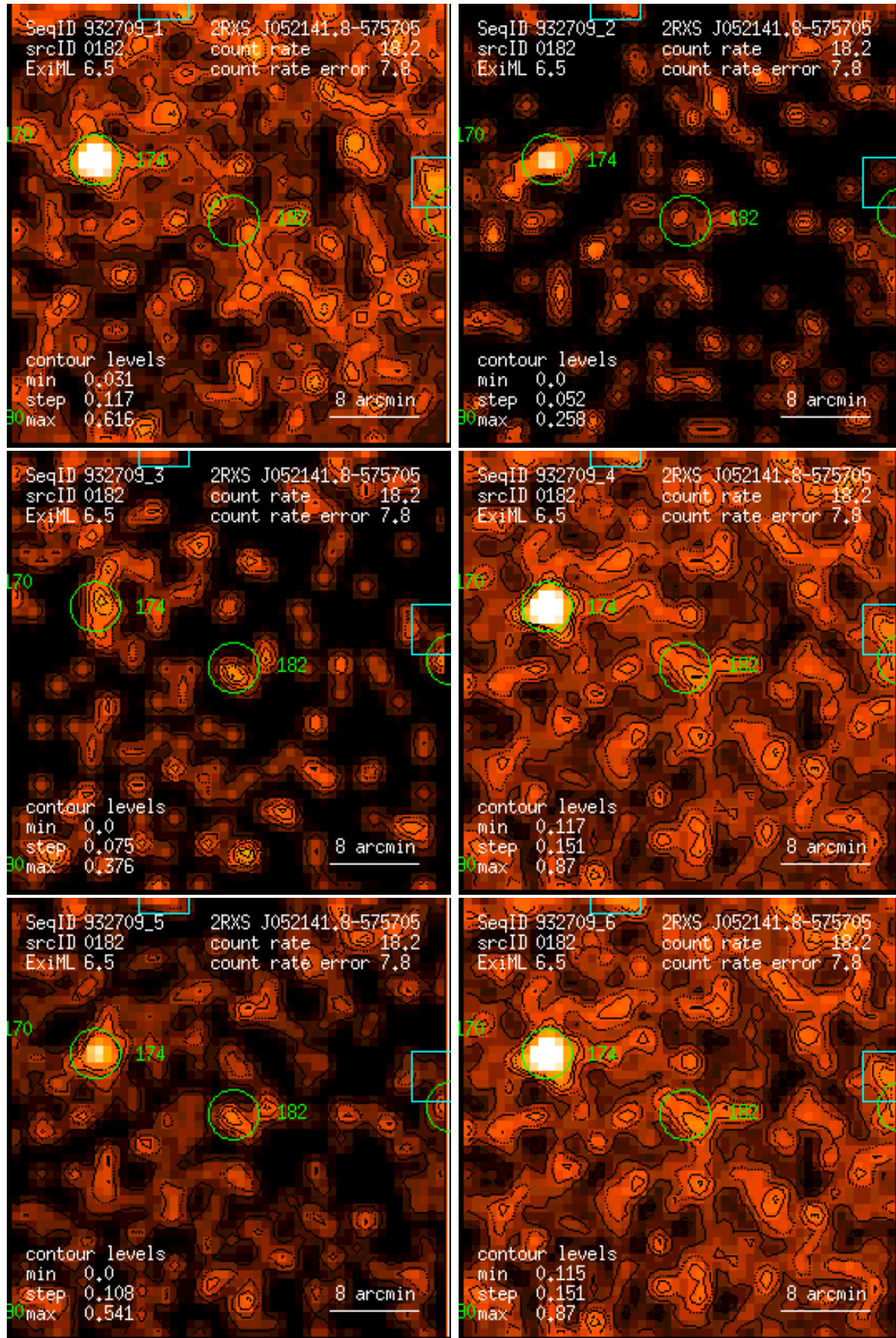
Figure 182: RASS 932709: detection 0182: band rate images, Gaussian filter: (1) PSPC channels 11 – 41, (2) 52 – 90, (3) 91 – 201, (4) 11 – 235, (5) 52 – 201, (6) 11 – 201. Broad band rates in counts/ks. Band rate contour levels in counts/ks/arcmin 2 .
