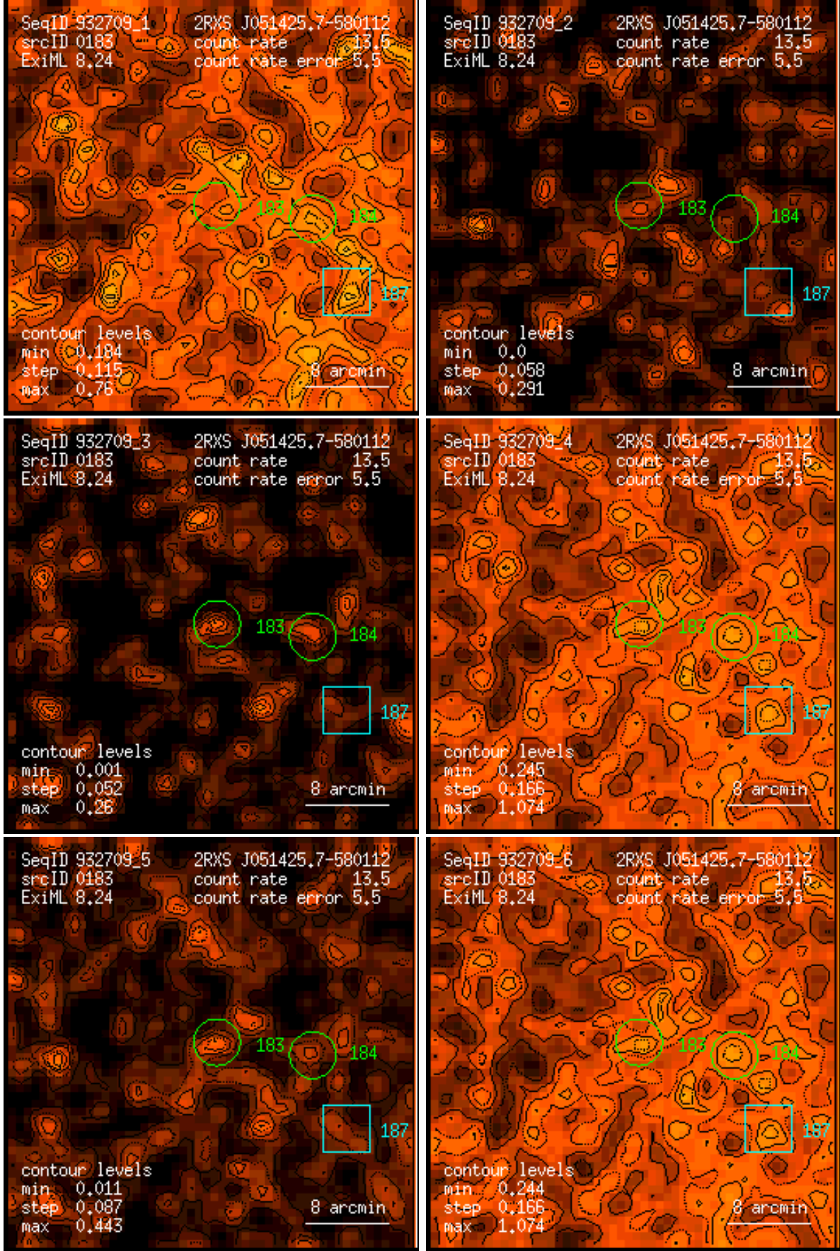
Figure 183: RASS 932709: detection 0183: band rate images, Gaussian filter: (1) PSPC channels 11 – 41, (2) 52 – 90, (3) 91 – 201, (4) 11 – 235, (5) 52 – 201, (6) 11 – 201. Broad band rates in counts/ks. Band rate contour levels in counts/ks/arcmin 2 .
