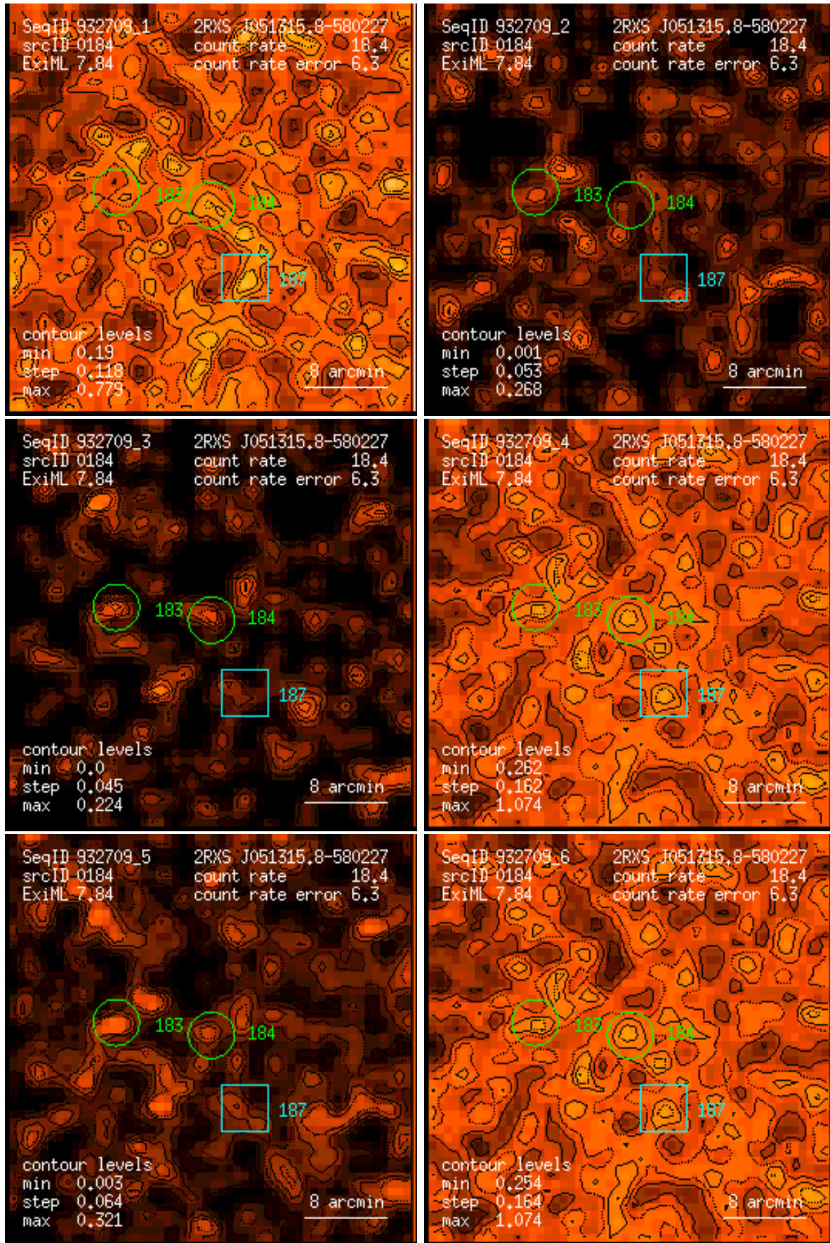
Figure 184: RASS 932709: detection 0184: band rate images, Gaussian filter: (1) PSPC channels 11 – 41, (2) 52 – 90, (3) 91 – 201, (4) 11 – 235, (5) 52 – 201, (6) 11 – 201. Broad band rates in counts/ks. Band rate contour levels in counts/ks/arcmin 2 .
