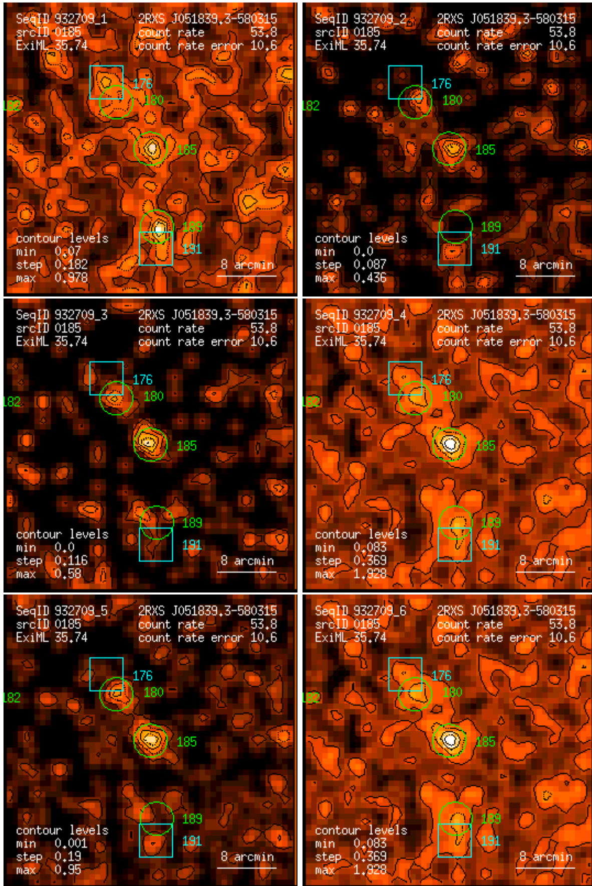
Figure 185: RASS 932709: detection 0185: band rate images, Gaussian filter: (1) PSPC channels 11 – 41, (2) 52 – 90, (3) 91 – 201, (4) 11 – 235, (5) 52 – 201, (6) 11 – 201. Broad band rates in counts/ks. Band rate contour levels in counts/ks/arcmin 2 .
