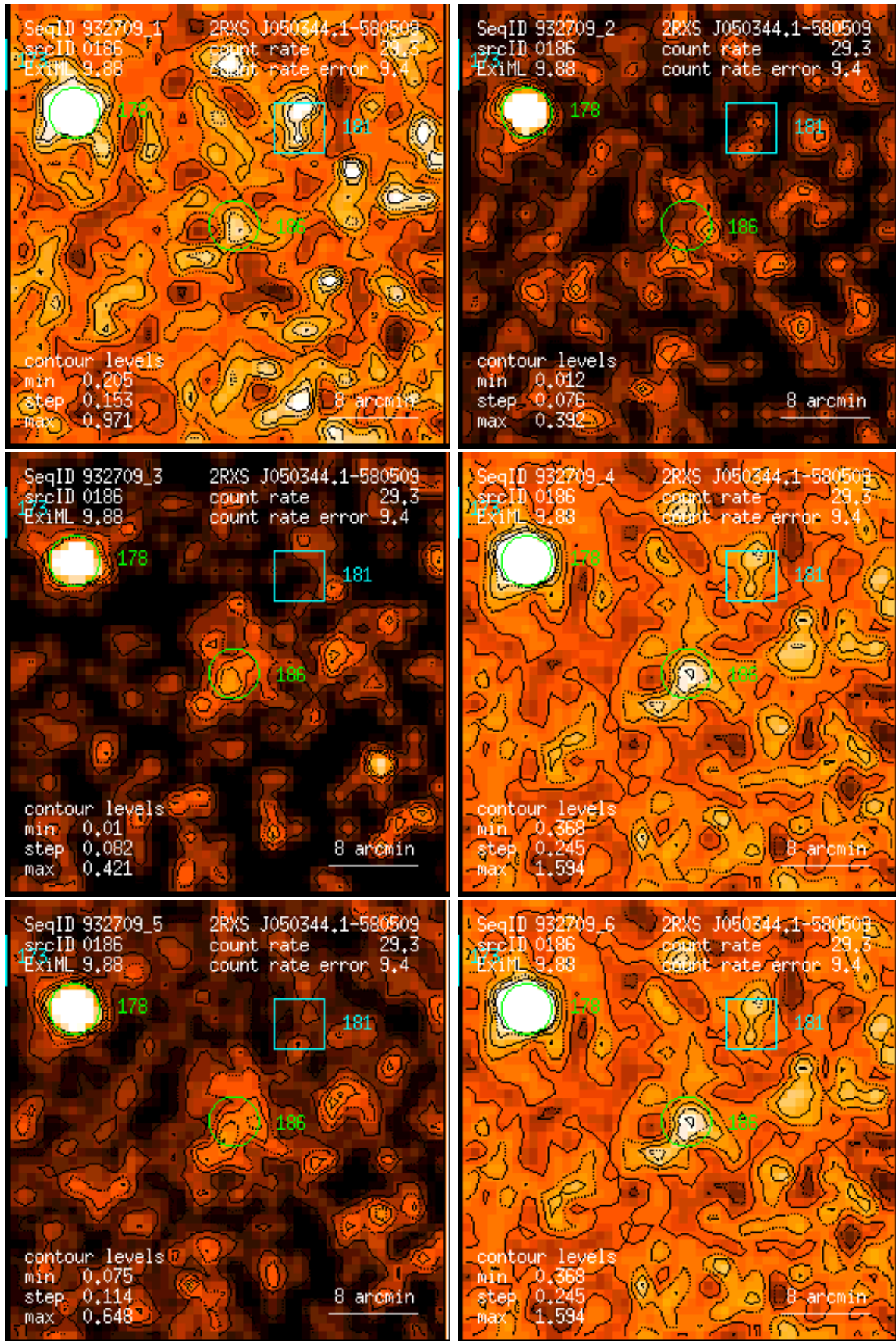
Figure 186: RASS 932709: detection 0186: band rate images, Gaussian filter: (1) PSPC channels 11 – 41, (2) 52 – 90, (3) 91 – 201, (4) 11 – 235, (5) 52 – 201, (6) 11 – 201. Broad band rates in counts/ks. Band rate contour levels in counts/ks/arcmin 2 .
