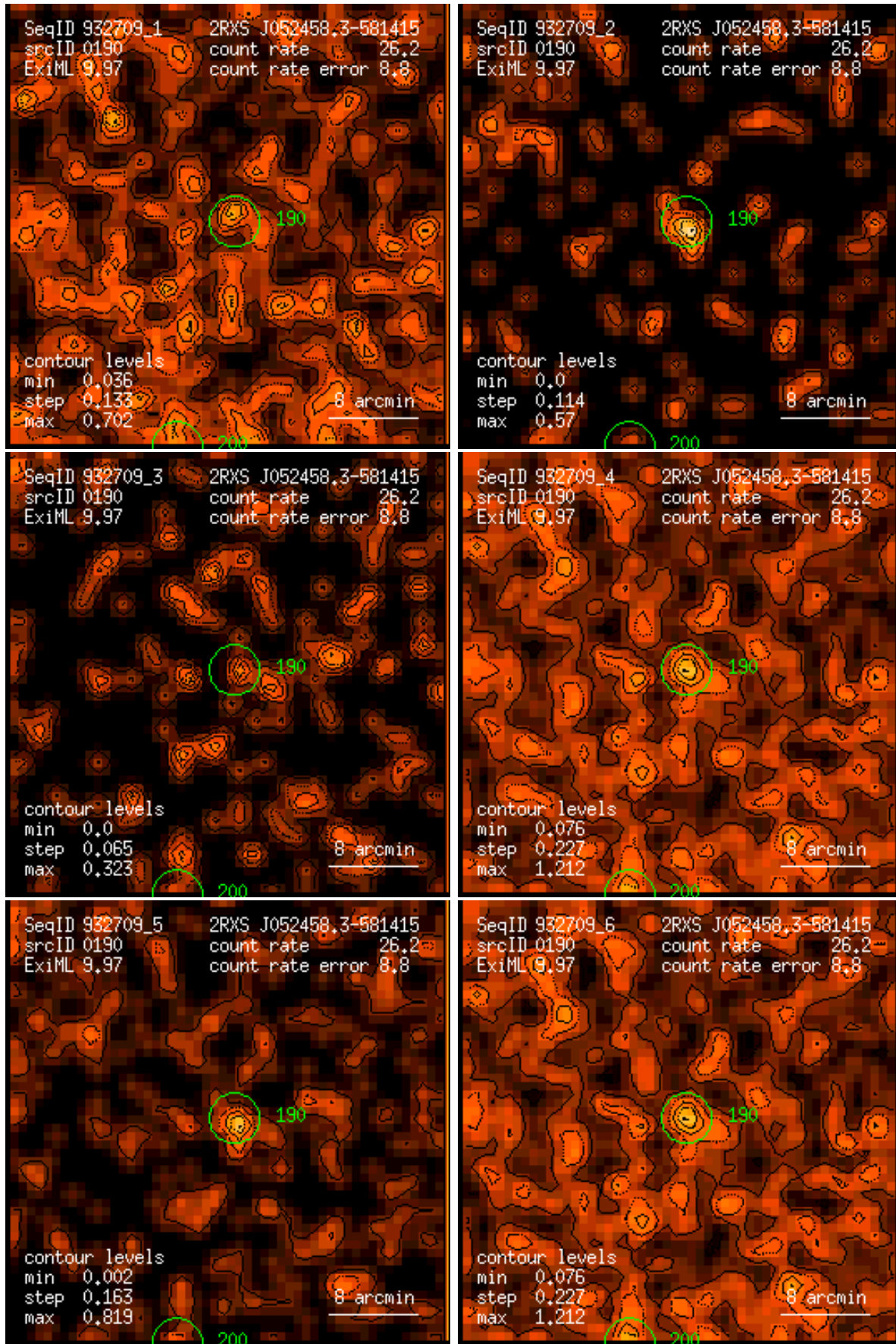
Figure 190: RASS 932709: detection 0190: band rate images, Gaussian filter: (1) PSPC channels 11 – 41, (2) 52 – 90, (3) 91 – 201, (4) 11 – 235, (5) 52 – 201, (6) 11 – 201. Broad band rates in counts/ks. Band rate contour levels in counts/ks/arcmin 2 .
