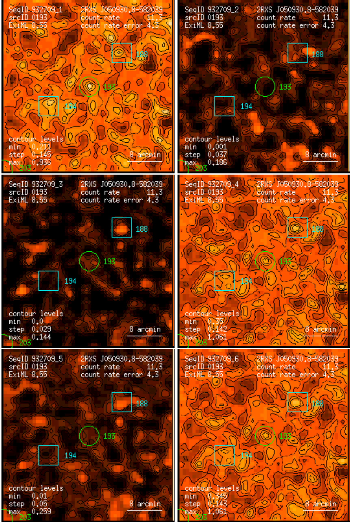
Figure 193: RASS 932709: detection 0193: band rate images, Gaussian filter: (1) PSPC channels 11 – 41, (2) 52 – 90, (3) 91 – 201, (4) 11 – 235, (5) 52 – 201, (6) 11 – 201. Broad band rates in counts/ks. Band rate contour levels in counts/ks/arcmin 2 .
