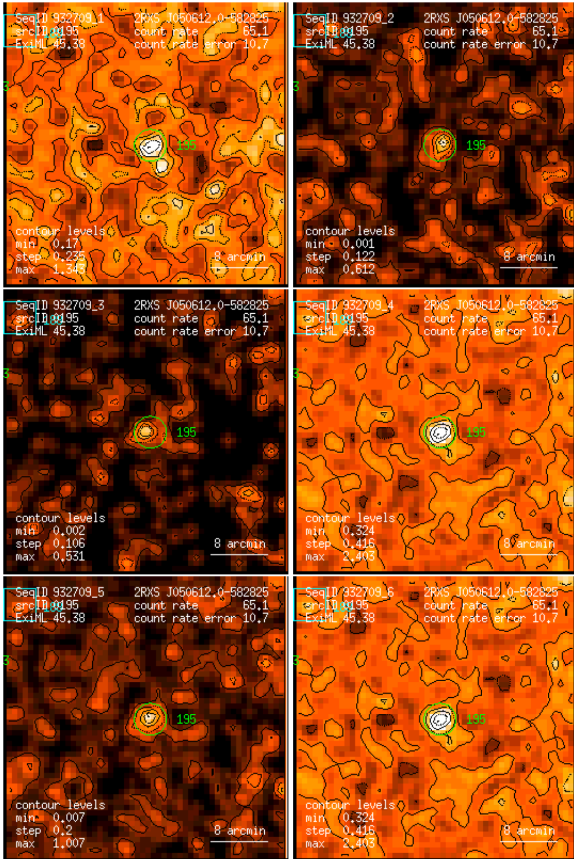
Figure 195: RASS 932709: detection 0195: band rate images, Gaussian filter: (1) PSPC channels 11 – 41, (2) 52 – 90, (3) 91 – 201, (4) 11 – 235, (5) 52 – 201, (6) 11 – 201. Broad band rates in counts/ks. Band rate contour levels in counts/ks/arcmin 2 .
