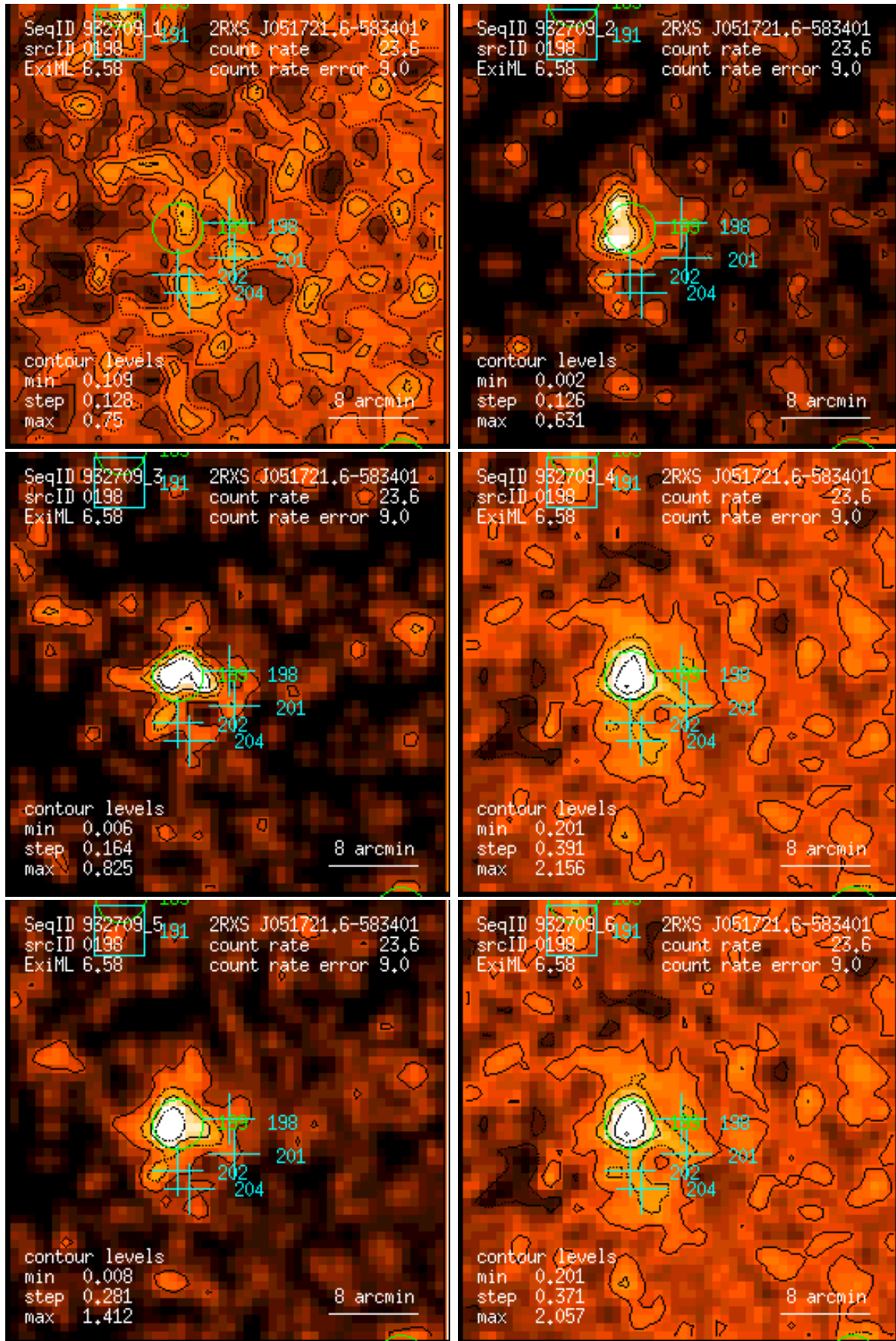
Figure 198: RASS 932709: detection 0198: band rate images, Gaussian filter: (1) PSPC channels 11 – 41, (2) 52 – 90, (3) 91 – 201, (4) 11 – 235, (5) 52 – 201, (6) 11 – 201. Broad band rates in counts/ks. Band rate contour levels in counts/ks/arcmin 2 .
