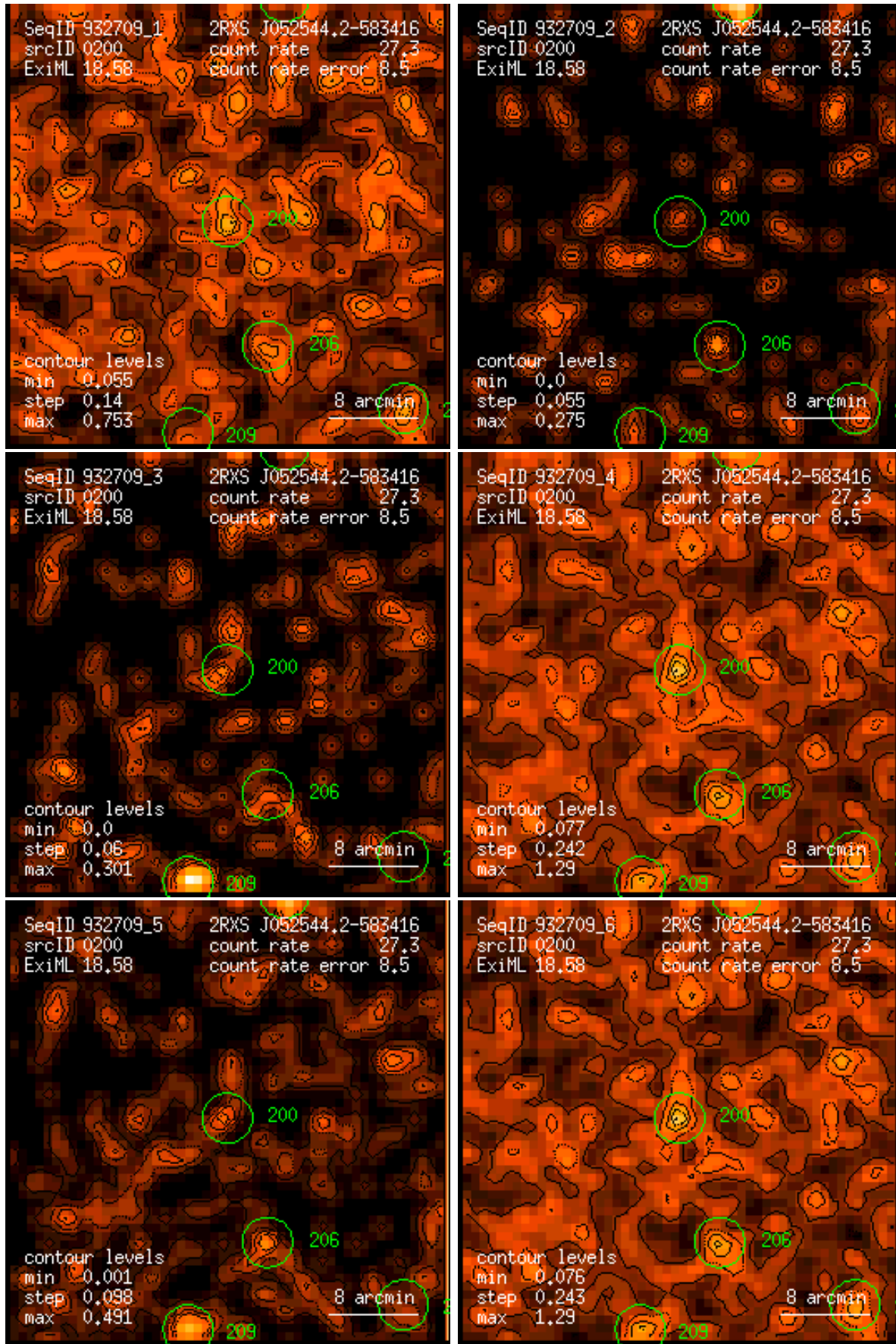
Figure 200: RASS 932709: detection 0200: band rate images, Gaussian filter: (1) PSPC channels 11 – 41, (2) 52 – 90, (3) 91 – 201, (4) 11 – 235, (5) 52 – 201, (6) 11 – 201. Broad band rates in counts/ks. Band rate contour levels in counts/ks/arcmin 2 .
