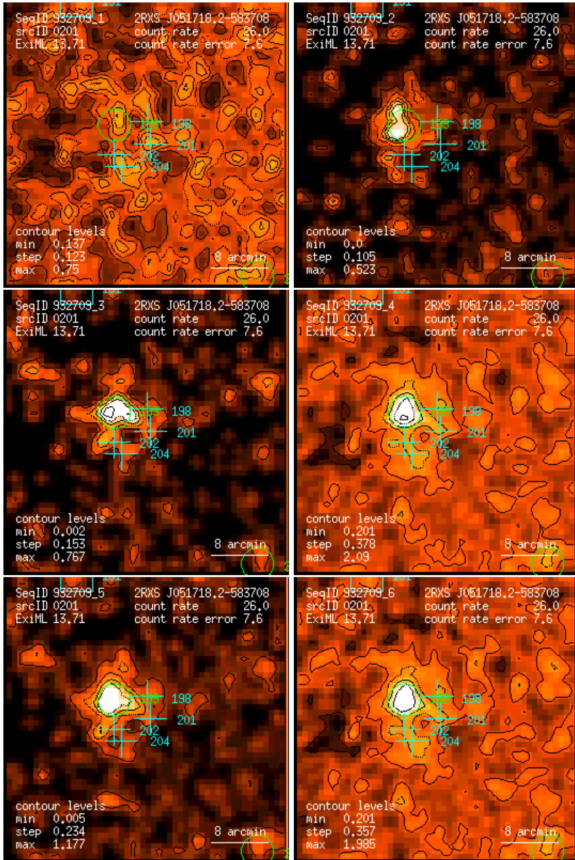
Figure 201: RASS 932709: detection 0201: band rate images, Gaussian filter: (1) PSPC channels 11 – 41, (2) 52 – 90, (3) 91 – 201, (4) 11 – 235, (5) 52 – 201, (6) 11 – 201. Broad band rates in counts/ks. Band rate contour levels in counts/ks/arcmin 2 .
