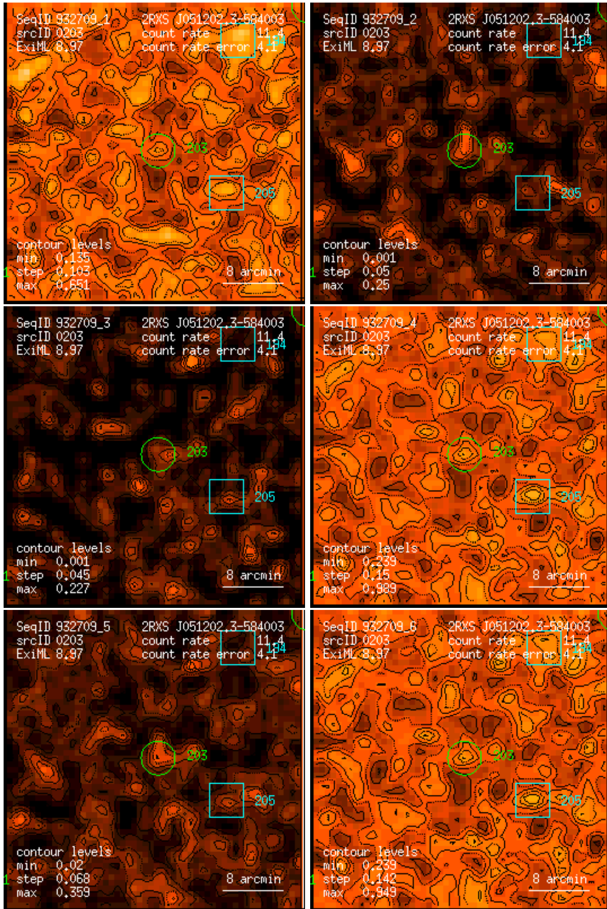
Figure 203: RASS 932709: detection 0203: band rate images, Gaussian filter: (1) PSPC channels 11 – 41, (2) 52 – 90, (3) 91 – 201, (4) 11 – 235, (5) 52 – 201, (6) 11 – 201. Broad band rates in counts/ks. Band rate contour levels in counts/ks/arcmin 2 .
