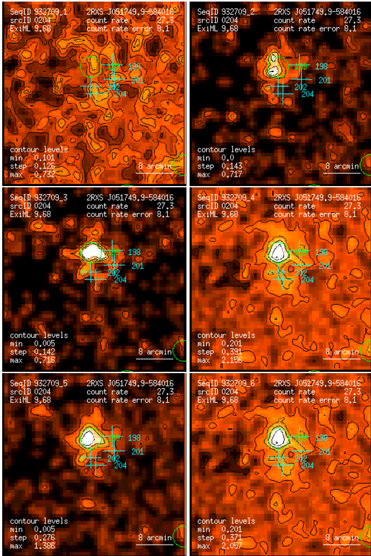
Figure 204: RASS 932709: detection 0204: band rate images, Gaussian filter: (1) PSPC channels 11 – 41, (2) 52 – 90, (3) 91 – 201, (4) 11 – 235, (5) 52 – 201, (6) 11 – 201. Broad band rates in counts/ks. Band rate contour levels in counts/ks/arcmin 2 .
