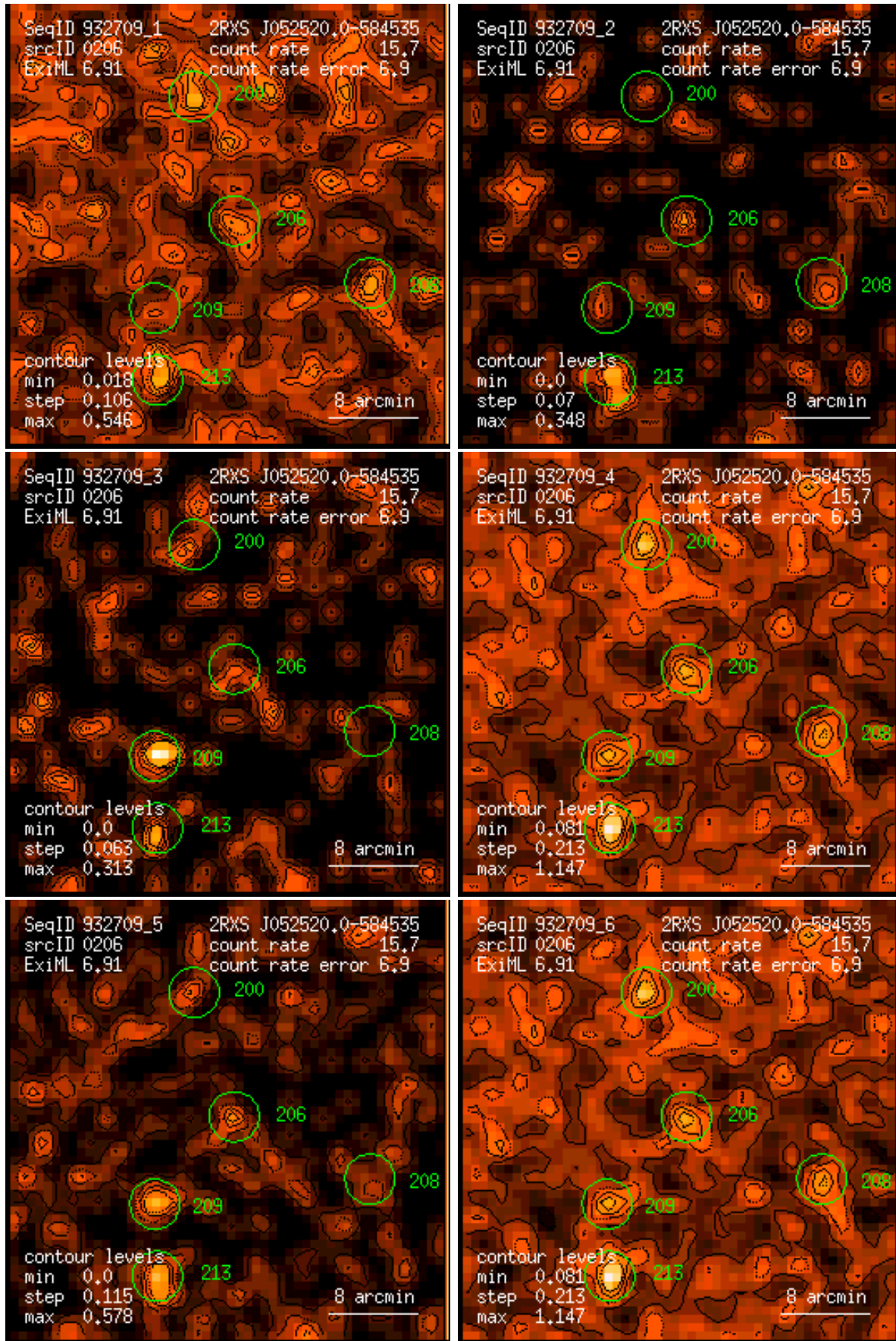
Figure 206: RASS 932709: detection 0206: band rate images, Gaussian filter: (1) PSPC channels 11 – 41, (2) 52 – 90, (3) 91 – 201, (4) 11 – 235, (5) 52 – 201, (6) 11 – 201. Broad band rates in counts/ks. Band rate contour levels in counts/ks/arcmin 2 .
