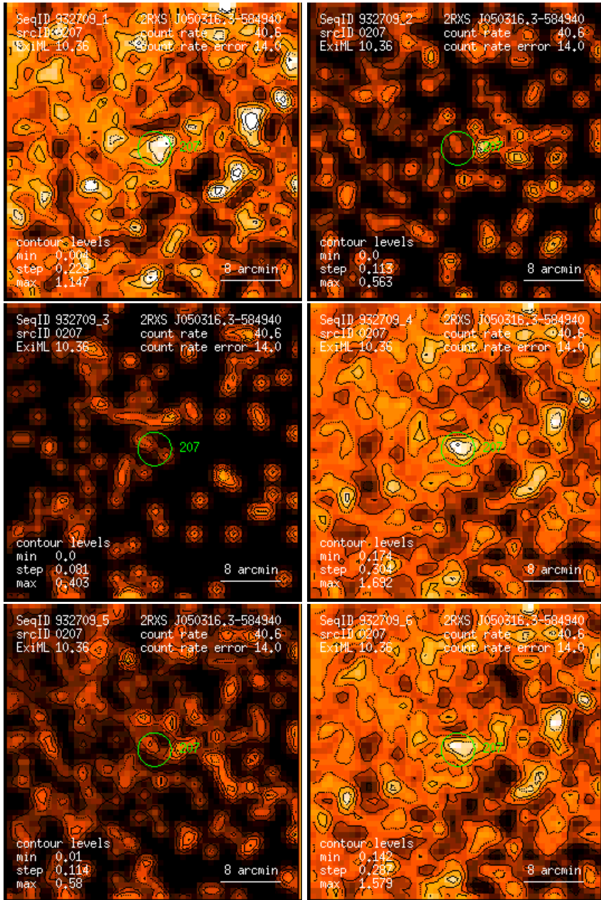
Figure 207: RASS 932709: detection 0207: band rate images, Gaussian filter: (1) PSPC channels 11 – 41, (2) 52 – 90, (3) 91 – 201, (4) 11 – 235, (5) 52 – 201, (6) 11 – 201. Broad band rates in counts/ks. Band rate contour levels in counts/ks/arcmin 2 .
