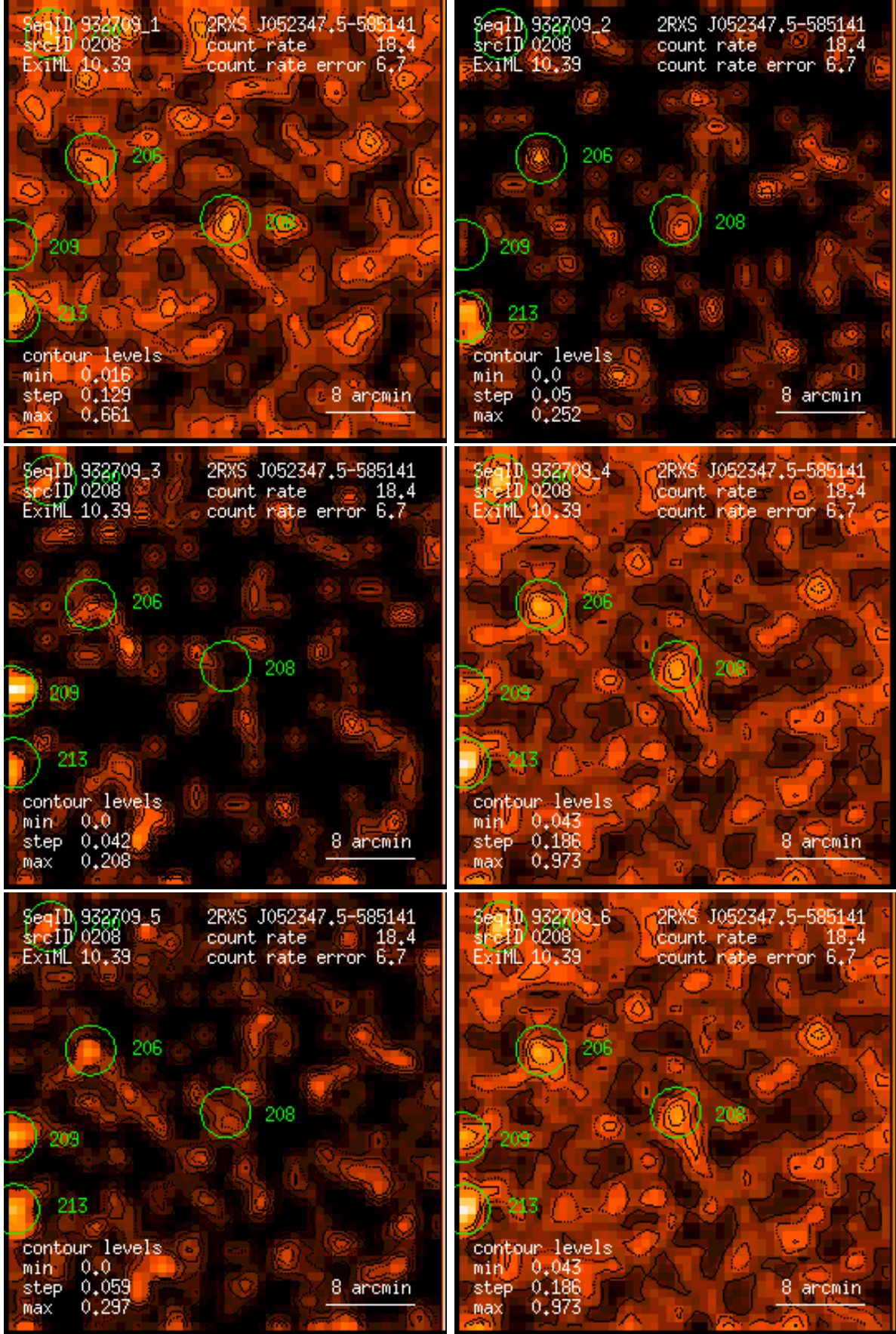
Figure 208: RASS 932709: detection 0208: band rate images, Gaussian filter: (1) PSPC channels 11 – 41, (2) 52 – 90, (3) 91 – 201, (4) 11 – 235, (5) 52 – 201, (6) 11 – 201. Broad band rates in counts/ks. Band rate contour levels in counts/ks/arcmin 2 .
