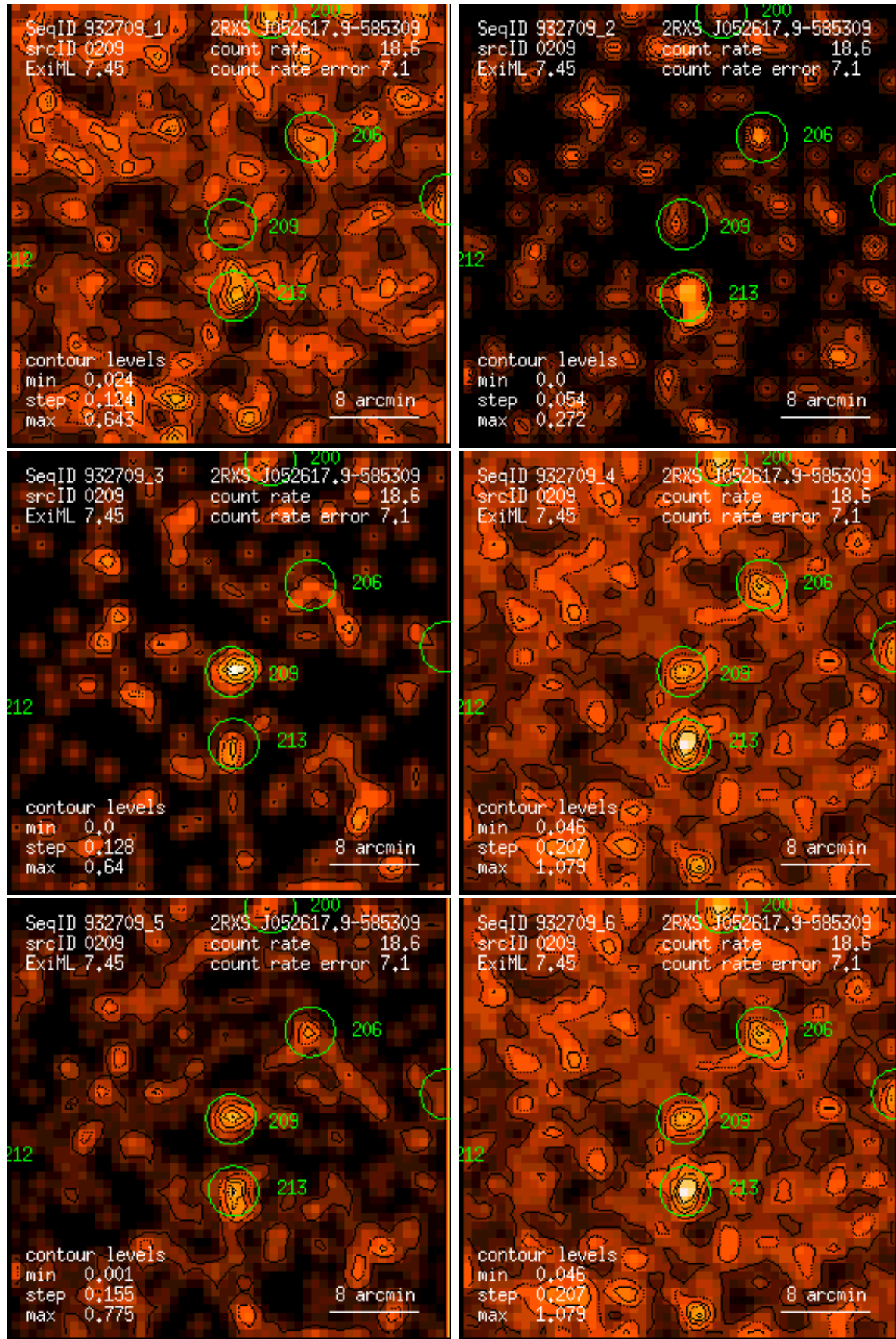
Figure 209: RASS 932709: detection 0209: band rate images, Gaussian filter: (1) PSPC channels 11 – 41, (2) 52 – 90, (3) 91 – 201, (4) 11 – 235, (5) 52 – 201, (6) 11 – 201. Broad band rates in counts/ks. Band rate contour levels in counts/ks/arcmin 2 .
