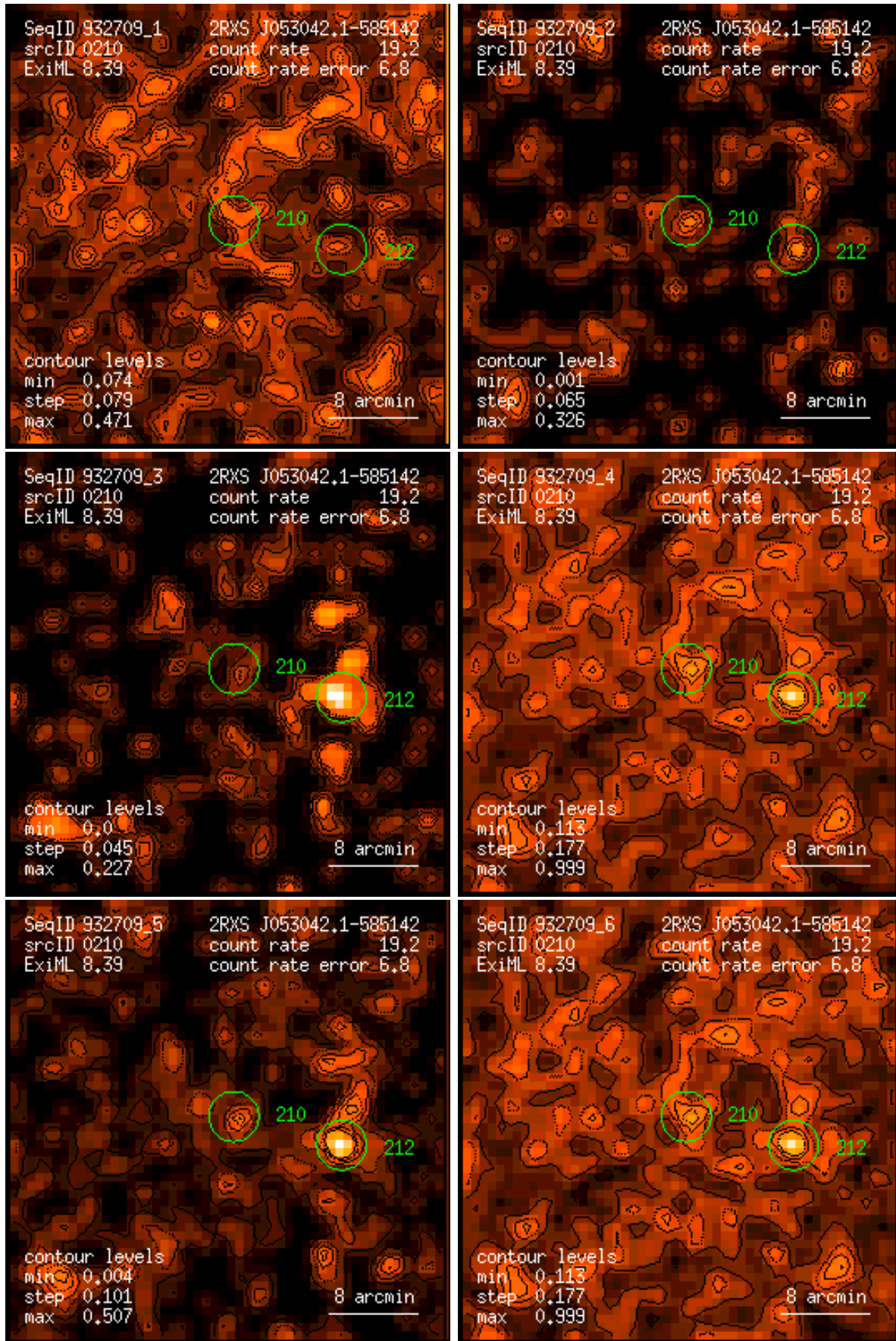
Figure 210: RASS 932709: detection 0210: band rate images, Gaussian filter: (1) PSPC channels 11 – 41, (2) 52 – 90, (3) 91 – 201, (4) 11 – 235, (5) 52 – 201, (6) 11 – 201. Broad band rates in counts/ks. Band rate contour levels in counts/ks/arcmin 2 .
