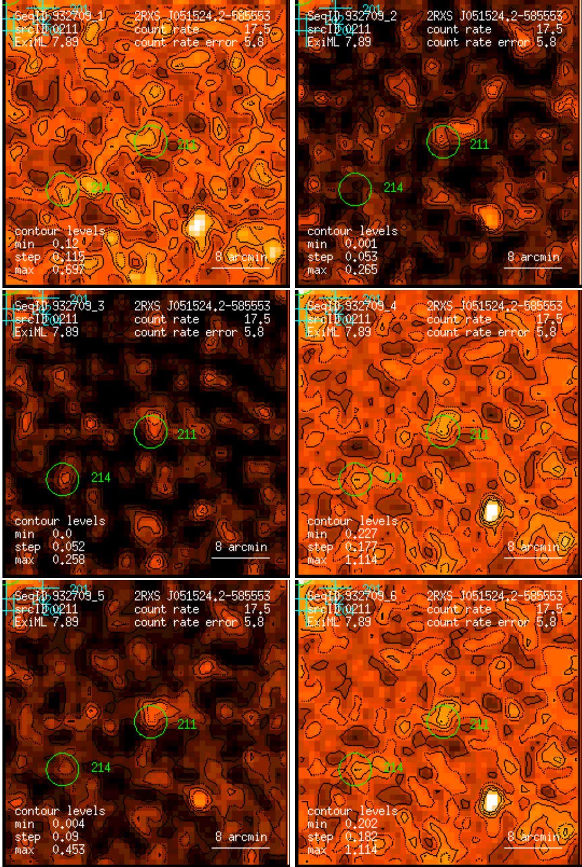
Figure 211: RASS 932709: detection 0211: band rate images, Gaussian filter: (1) PSPC channels 11 – 41, (2) 52 – 90, (3) 91 – 201, (4) 11 – 235, (5) 52 – 201, (6) 11 – 201. Broad band rates in counts/ks. Band rate contour levels in counts/ks/arcmin 2 .
